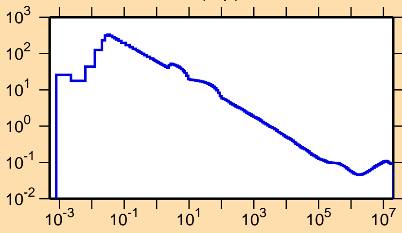
\sigma vs. E for ^{168}\text{Ta}(n,p)
