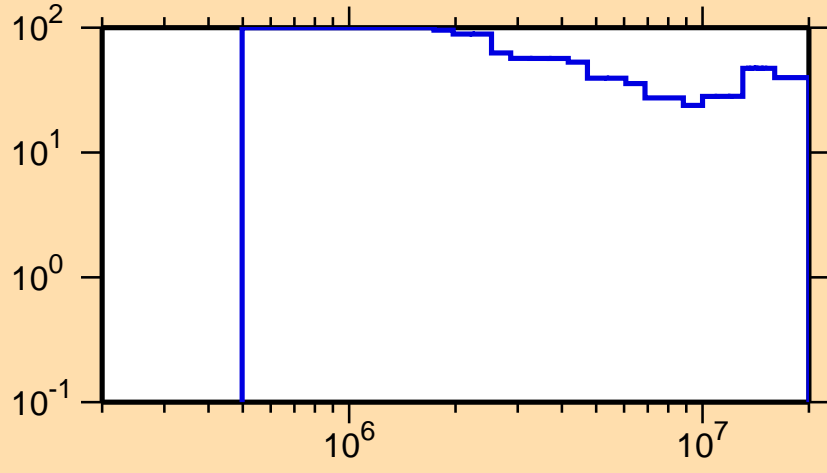
\Delta\sigma/\sigma vs. E for ^{168}\text{Ta}(n,n\text{cont.})
