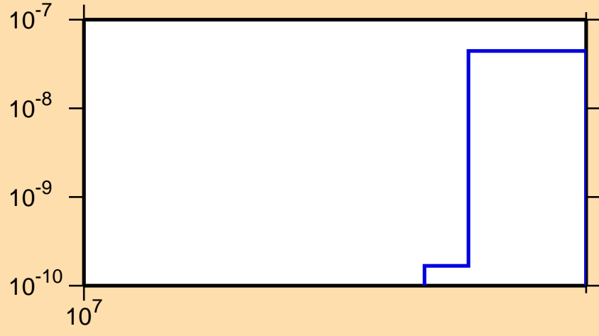
\sigma vs. E for ^{168}\text{Ta}(n,nt)
