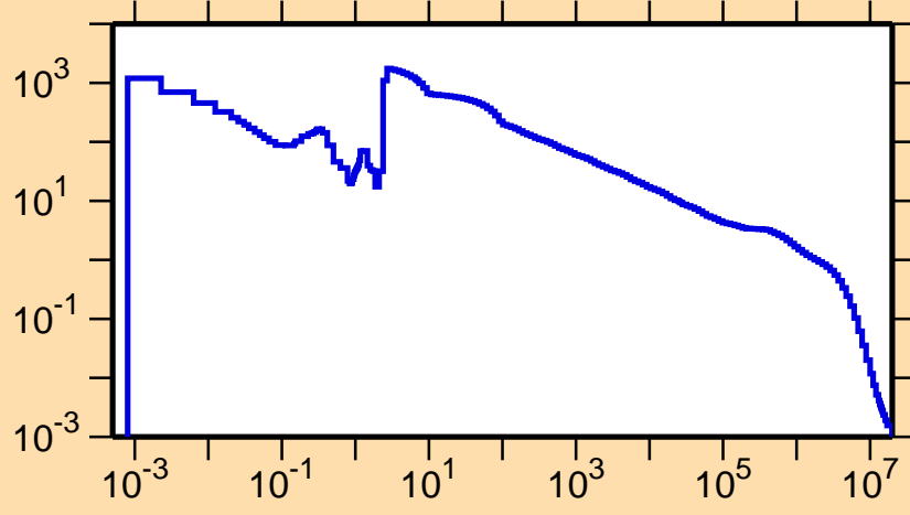
\sigma vs. E for ^{168}\text{Ta}(n,\gamma)
