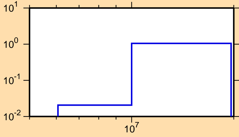
\sigma vs. E for ^{168}\text{Ta}(n,2n)
