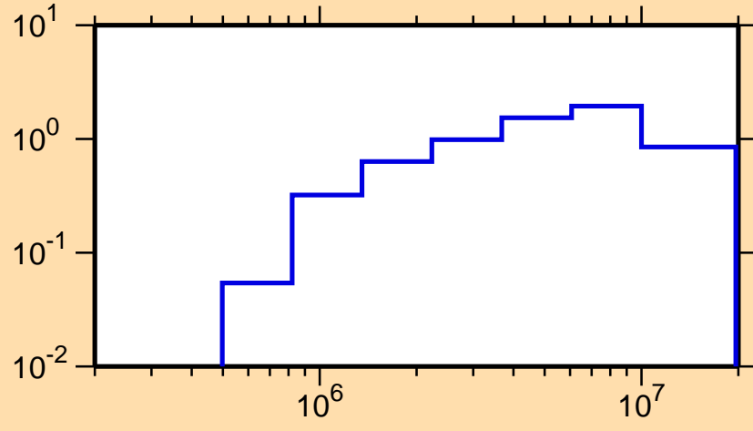
\sigma vs. E for ^{168}\text{Ta}(n,n\text{cont.})
