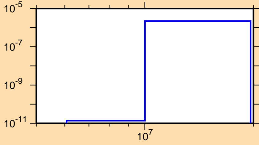
\sigma vs. E for ^{168}\text{Ta}(n,\text{He3})
