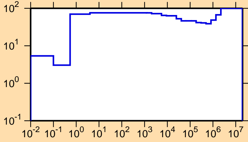
\Delta\sigma/\sigma vs. E for ^{168}\text{Ta}(n,\gamma)
