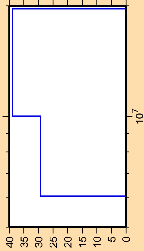
\Delta\sigma/\sigma vs. E for ^{168}\text{Ta}(n,n\text{cont.})
