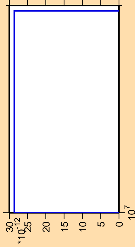
\Delta\sigma/\sigma vs. E for ^{168}\text{Ta} (mt 11)
