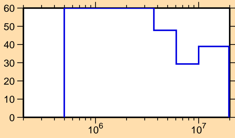
\Delta\sigma/\sigma vs. E for ^{168}\text{Ta}(n,n\text{cont.})
