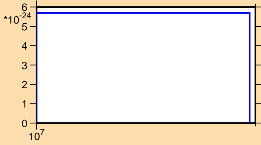
\sigma vs. E for ^{168}\text{Ta} (mt 11)
