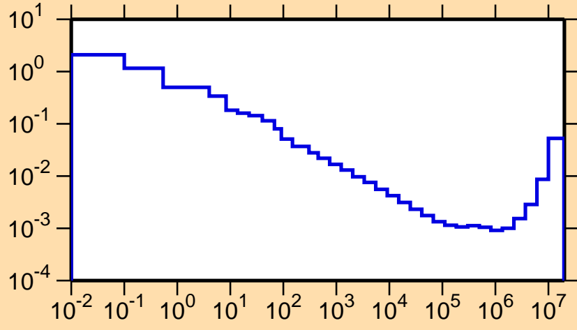
\sigma vs. E for ^{168}\text{Ta}(n,\alpha)
