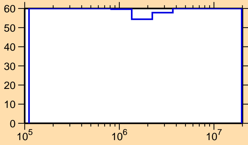
\Delta\sigma/\sigma vs. E for ^{168}\text{Ta}(n,n_1)
