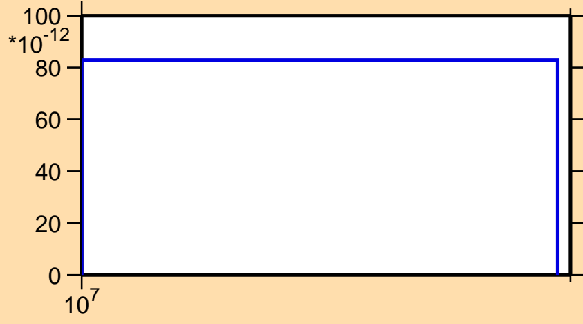
\sigma vs. E for ^{168}\text{Ta}(n,\text{pt})
