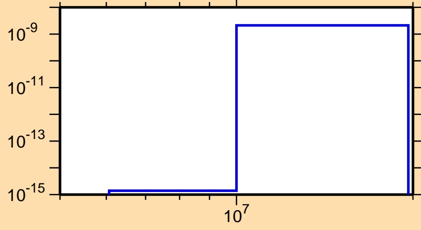
\sigma vs. E for ^{168}\text{Ta}(\text{mt117})
