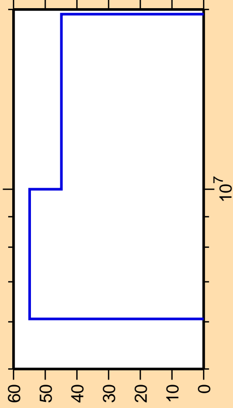
\Delta\sigma/\sigma vs. E for ^{168}\text{Ta}(n,2n)
