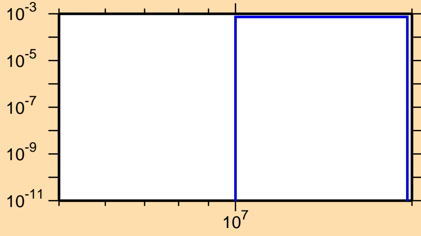
\sigma vs. E for ^{168}\text{Ta}(n,2np)
