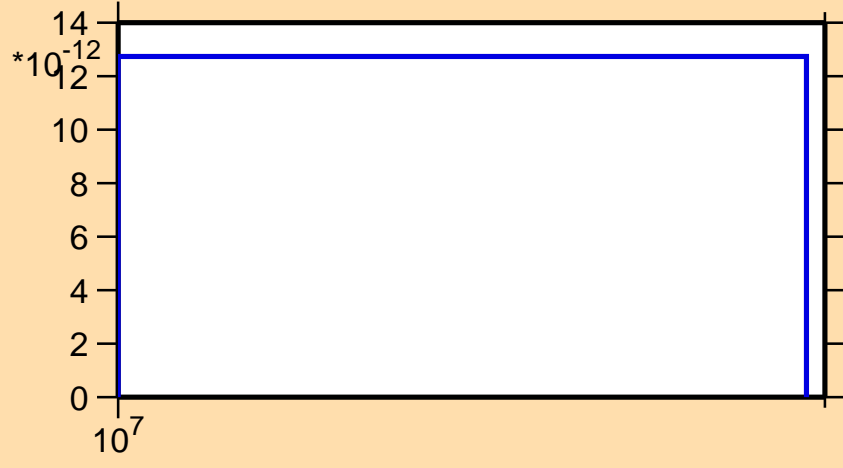
\sigma vs. E for ^{168}\text{Ta} (mt 34)
