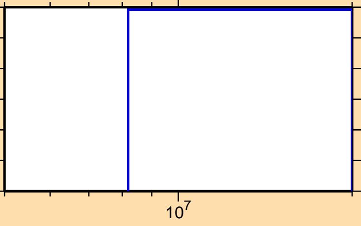
\sigma vs. E for ^{168}\text{Ta}(n,2np)
