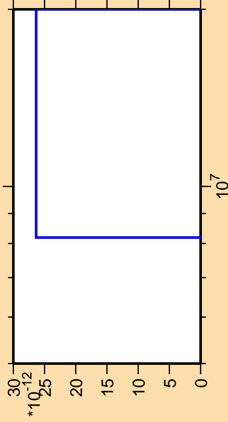
\Delta\sigma/\sigma vs. E for ^{168}\text{Ta}(\text{mt } 11)
