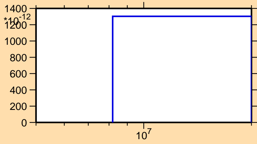
\sigma vs. E for ^{168}\text{Ta}(n,pd)
