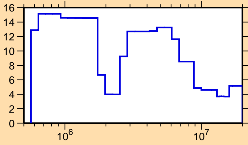
\Delta\sigma/\sigma vs. E for ^{169}\text{Ta}(n,tot.)
