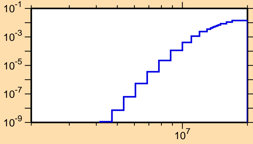
\sigma vs. E for ^{169}\text{Ta}(n,d)
