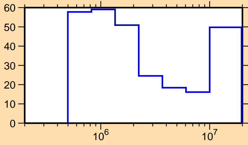
\Delta\sigma/\sigma vs. E for ^{169}\text{Ta}(n,n\text{cont.})
