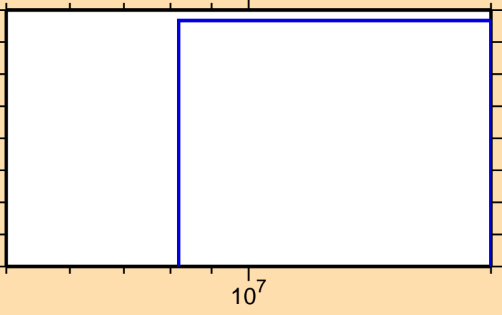
\sigma vs. E for ^{169}\text{Ta}(n,2np)
