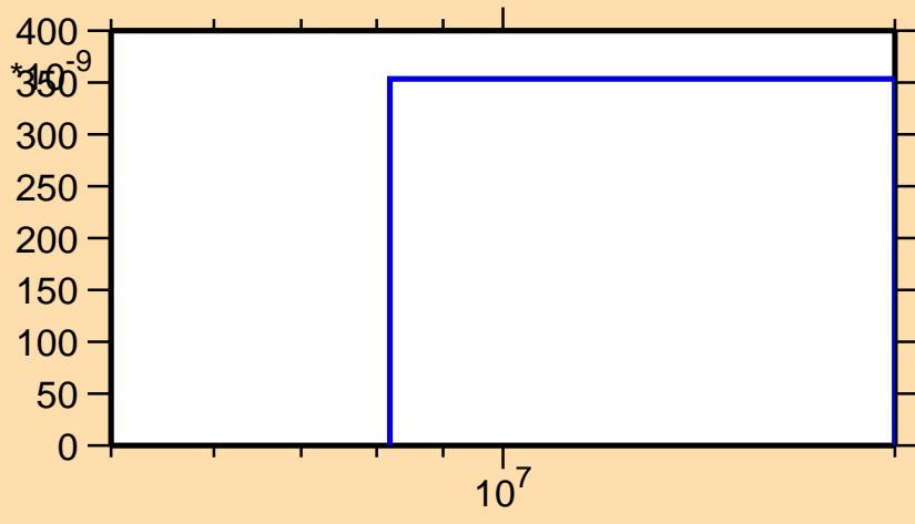
\sigma vs. E for ^{169}\text{Ta}(n,\text{He}3)
