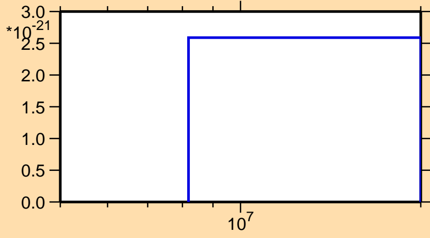
\sigma vs. E for ^{169}\text{Ta} (mt 42)
