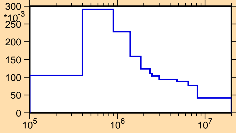
\sigma vs. E for ^{169}\text{Ta}(n,n_4)
