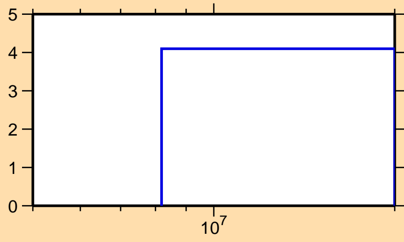
\Delta\sigma/\sigma vs. E for ^{169}\text{Ta}(n,\text{tot.})
