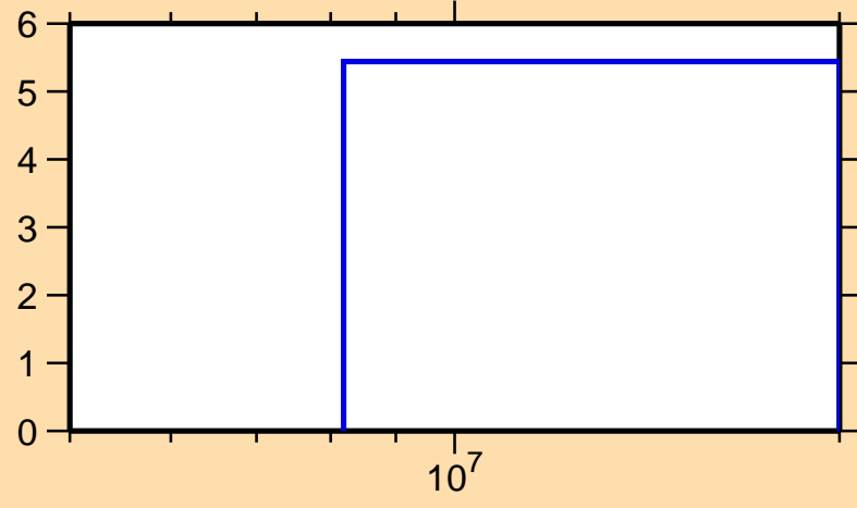
\Delta\sigma/\sigma vs. E for ^{169}\text{Ta}(n,\text{el.})
