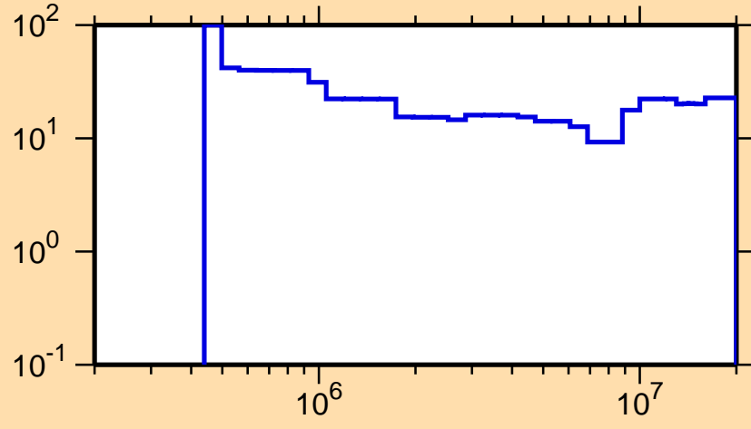
\Delta\sigma/\sigma vs. E for ^{170}\text{Ta}(n,n\text{cont.})
