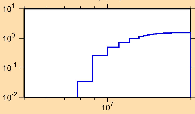
\sigma vs. E for ^{170}\text{Ta}(n,2n)
