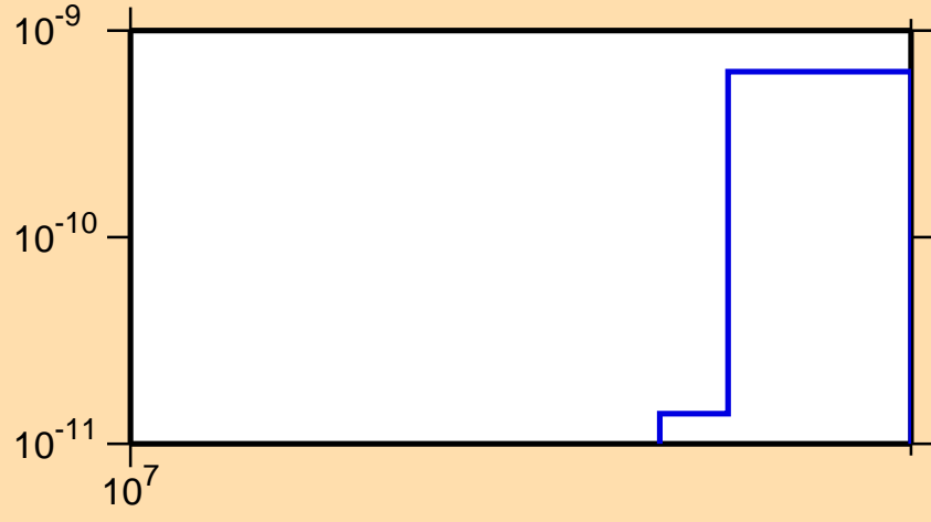
\sigma vs. E for ^{170}\text{Ta}(n,\text{pt})
