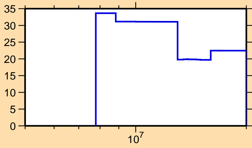
\Delta\sigma/\sigma vs. E for ^{170}\text{Ta}(n,2n)
