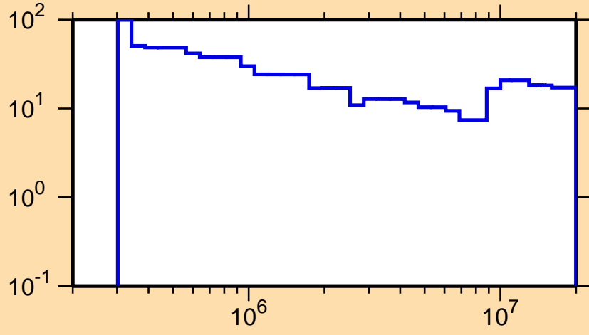
\Delta\sigma/\sigma vs. E for ^{170}\text{Ta}(n,inel.)
