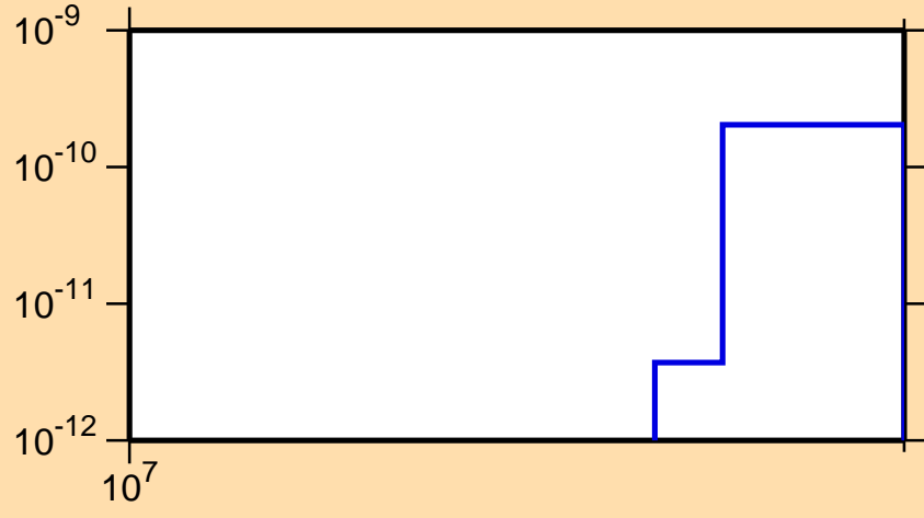
\sigma vs. E for ^{170}\text{Ta} (mt 34)
