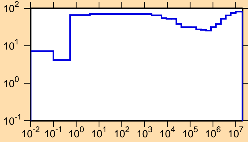
\Delta\sigma/\sigma vs. E for ^{170}\text{Ta}(n,\gamma)
