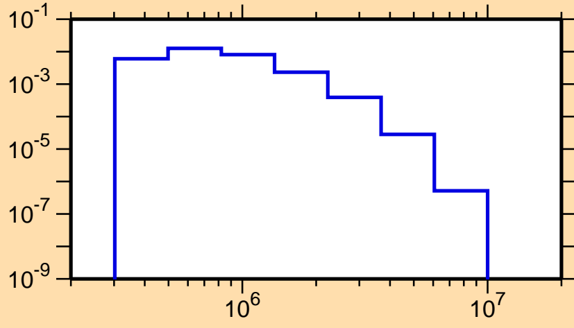
\sigma vs. E for ^{170}\text{Ta}(n,n_1)
