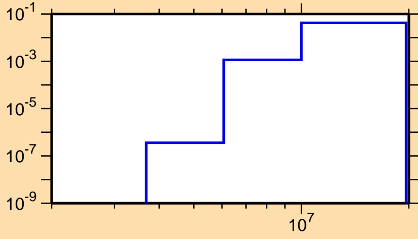
\sigma vs. E for ^{170}\text{Ta}(n,np)
