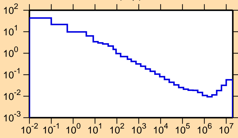
\sigma vs. E for ^{170}\text{Ta}(n,p)
