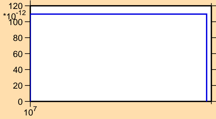
\sigma vs. E for ^{170}\text{Ta}(n,pd)
