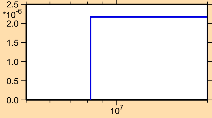
\sigma vs. E for ^{170}\text{Ta}(n,\text{nd})
