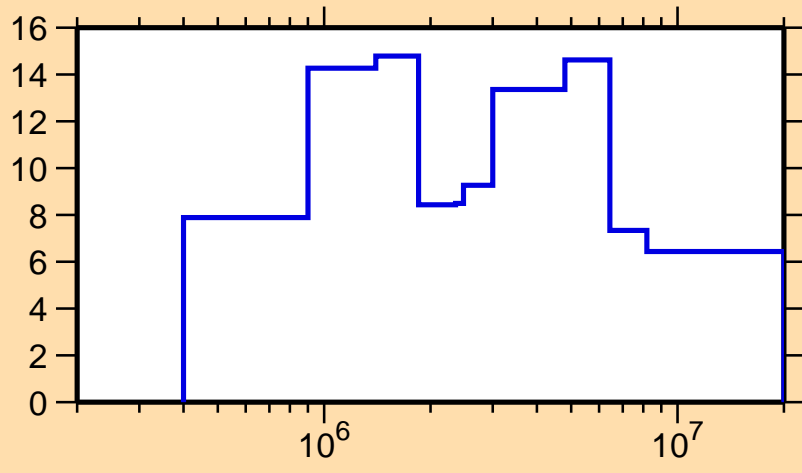
\Delta\sigma/\sigma vs. E for ^{170}\text{Ta}(n, el.)
