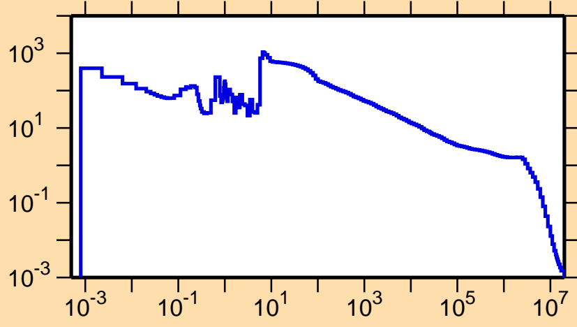
\sigma vs. E for ^{171}\text{Ta}(n,\gamma)
