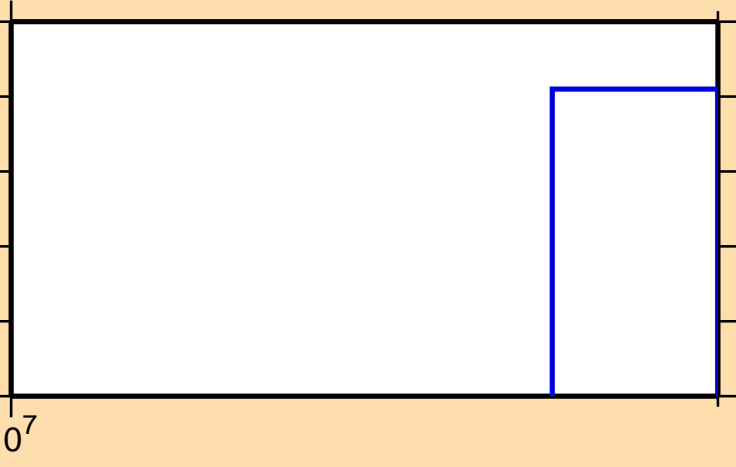
\sigma vs. E for ^{171}\text{Ta}(n,3n)
