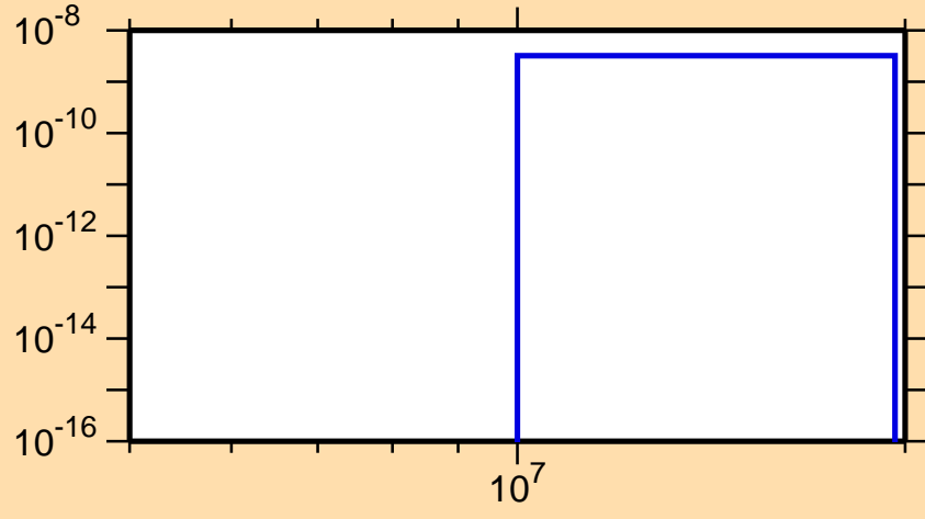
\sigma vs. E for ^{171}\text{Ta}(\text{mt } 45)
