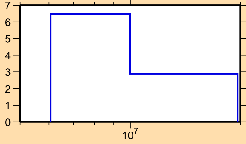
\Delta\sigma/\sigma vs. E for ^{171}\text{Ta}(n,\text{tot.})
