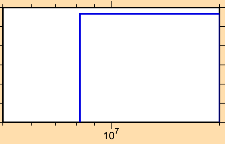
\sigma vs. E for ^{171}\text{Ta}(n,2n\alpha)
