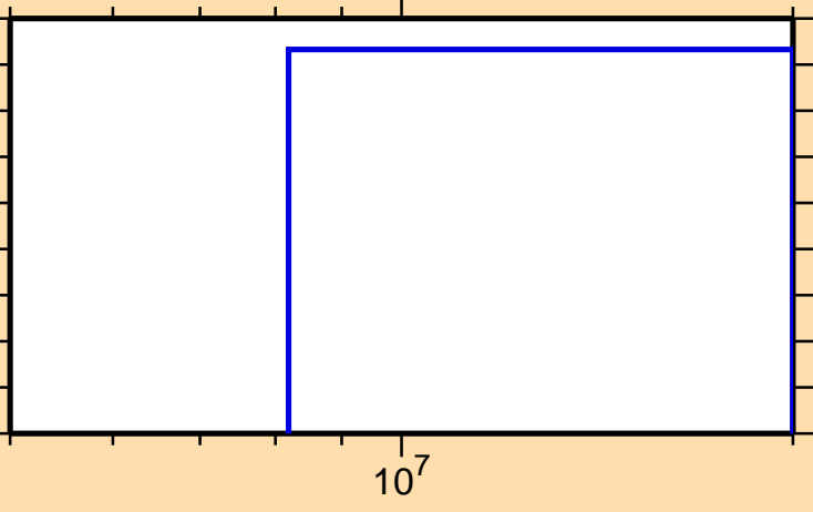
\sigma vs. E for ^{171}\text{Ta}(n,3n)
