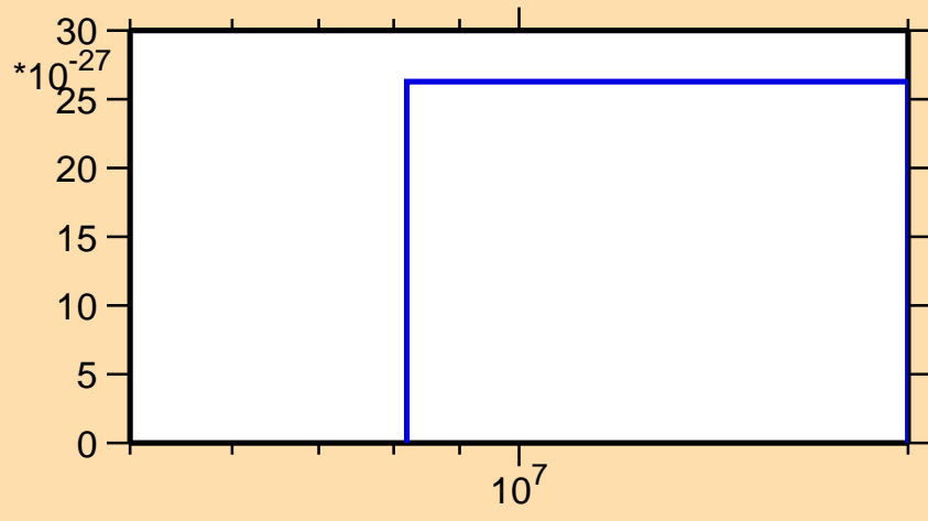
\sigma vs. E for ^{171}\text{Ta} (mt 42)
