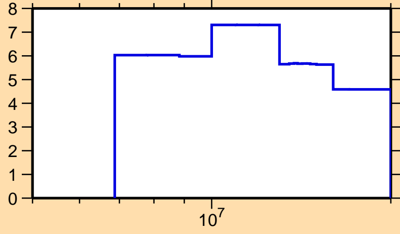
\Delta\sigma/\sigma vs. E for ^{172}\text{Ta}(n,\text{el.})
