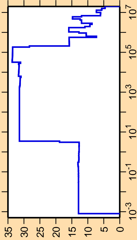
\Delta\sigma/\sigma vs. E for ^{172}\text{Ta}(n,\text{el.})
