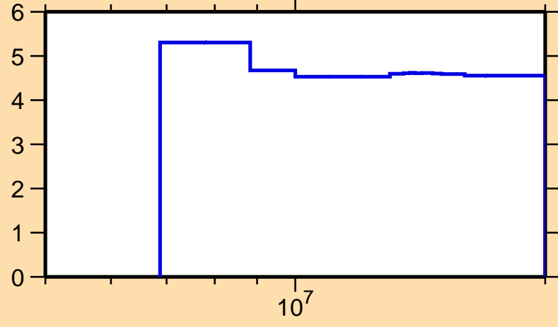
\Delta\sigma/\sigma vs. E for ^{172}\text{Ta}(n,\text{nonel.})
