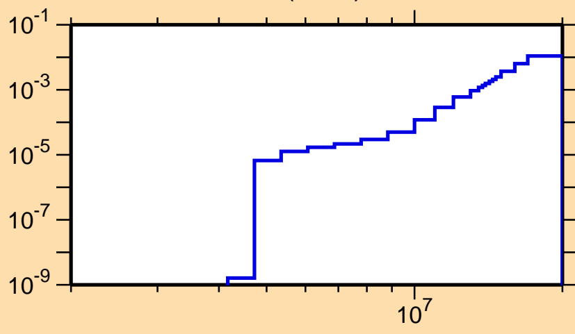
\sigma vs. E for ^{172}\text{Ta}(n,n\alpha)
