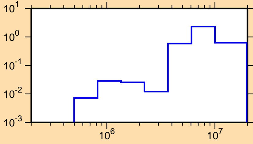
\sigma vs. E for ^{172}\text{Ta}(n,n\text{cont.})
