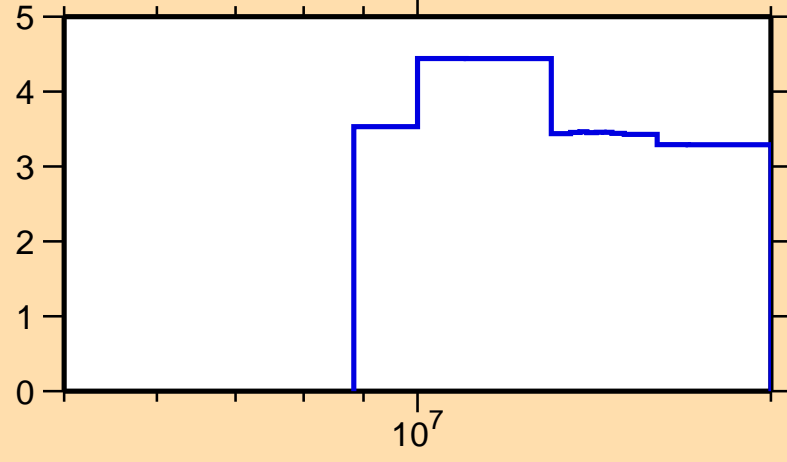
\Delta\sigma/\sigma vs. E for ^{173}\text{Ta}(n,\text{el.})
