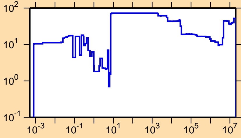
\Delta\sigma/\sigma vs. E for ^{173}\text{Ta}(n,\gamma)
