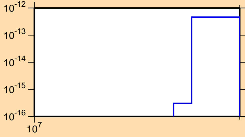
\sigma vs. E for ^{173}\text{Ta} (mt 34)
