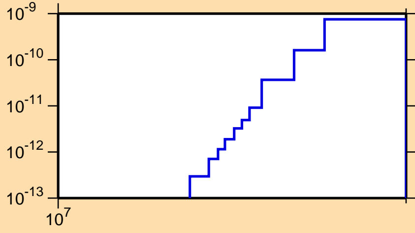
\sigma vs. E for ^{173}\text{Ta}(\text{mt117})
