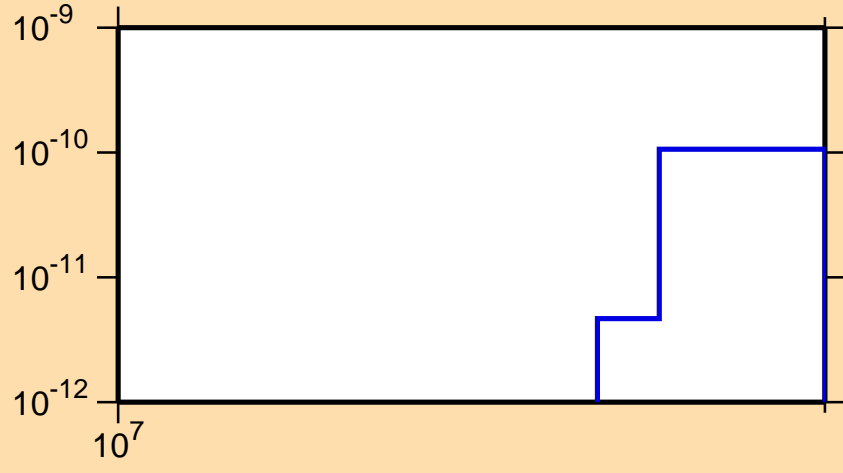
\sigma vs. E for ^{173}\text{Ta}(n,pd)
