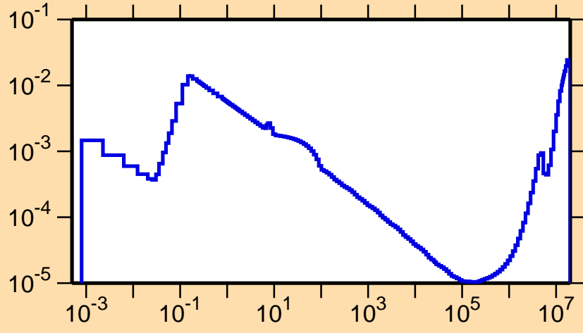
\sigma vs. E for ^{173}\text{Ta}(n,\alpha)
