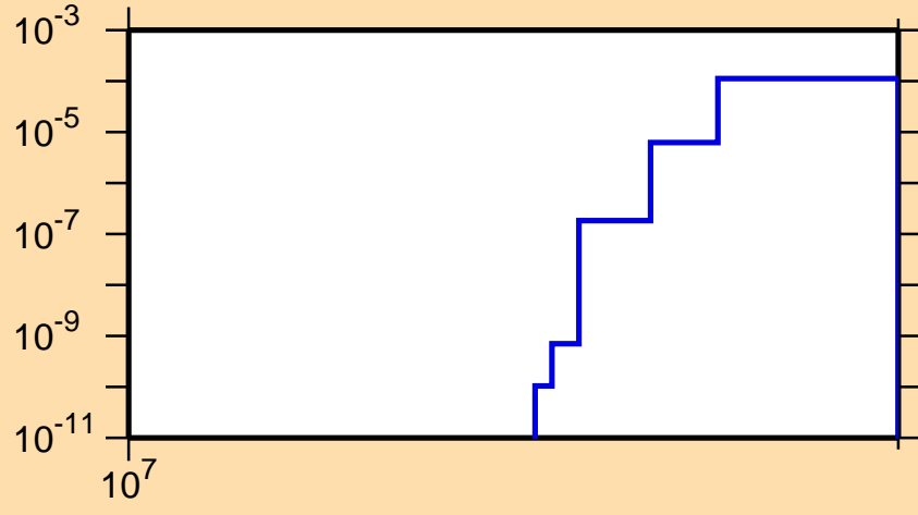
\sigma vs. E for ^{173}\text{Ta}(n,2np)
