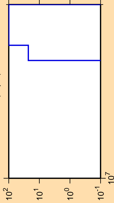
\Delta\sigma/\sigma vs. E for ^{173}\text{Ta}(n,pd)
