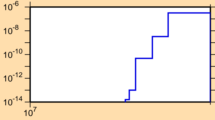
\sigma vs. E for ^{173}\text{Ta}(n,nt)
