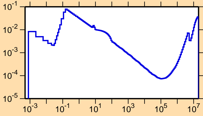
\sigma vs. E for ^{173}\text{Ta}(n,p)
