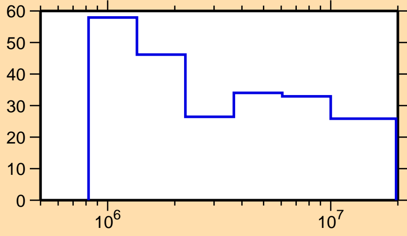
\Delta\sigma/\sigma vs. E for ^{173}\text{Ta}(n,n_1)
