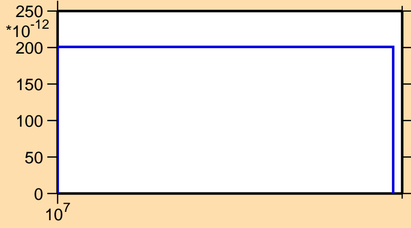
\sigma vs. E for ^{173}\text{Ta} (mt 45)
