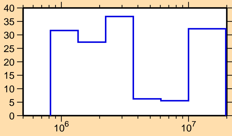
\Delta\sigma/\sigma vs. E for ^{173}\text{Ta}(n,n\text{cont.})
