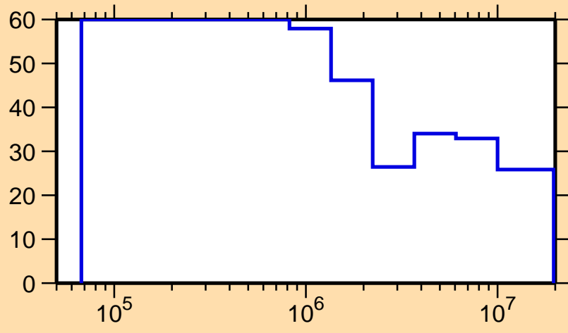
\Delta\sigma/\sigma vs. E for ^{173}\text{Ta}(n,n_1)
