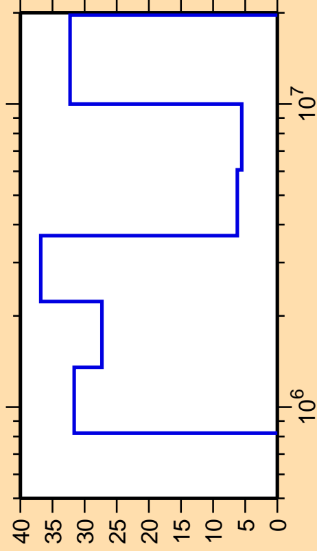
\Delta\sigma/\sigma vs. E for ^{173}\text{Ta}(n,\text{ncont.})
