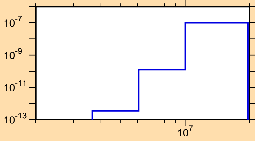
\sigma vs. E for ^{173}\text{Ta}(n,p\alpha)
