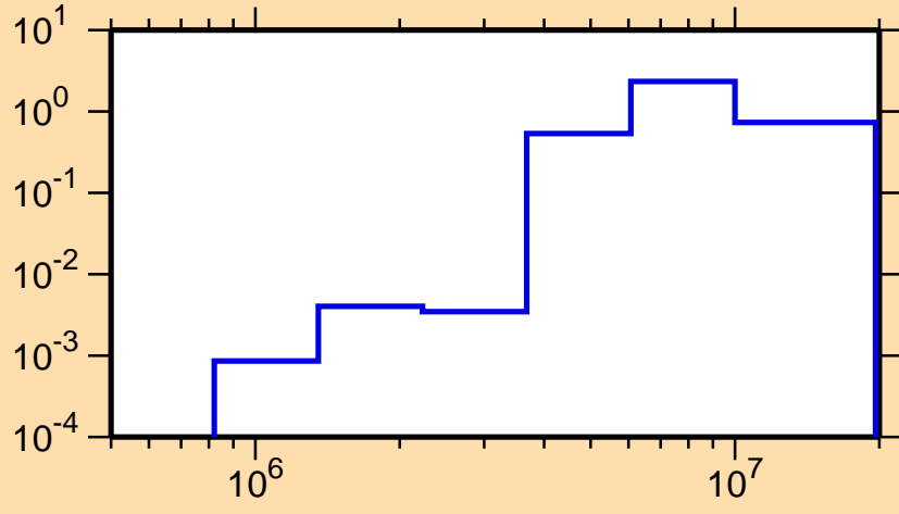
\sigma vs. E for ^{173}\text{Ta}(n,n\text{cont.})
