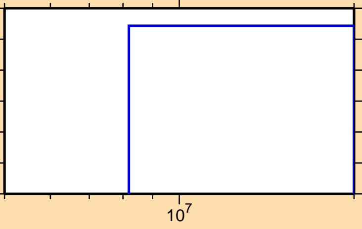
\sigma vs. E for ^{173}\text{Ta}(n,nt)
