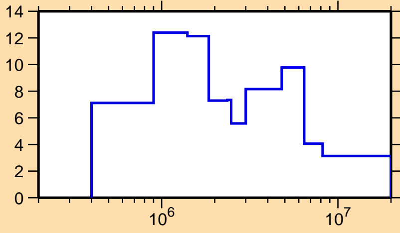
\Delta\sigma/\sigma vs. E for ^{173}\text{Ta}(n,el.)
