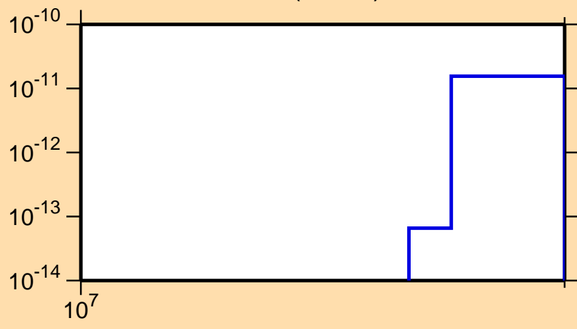
\sigma vs. E for ^{174}\text{Ta} (mt 34)
