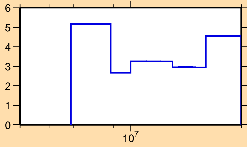
\Delta\sigma/\sigma vs. E for ^{174}\text{Ta}(n,\text{el.})
