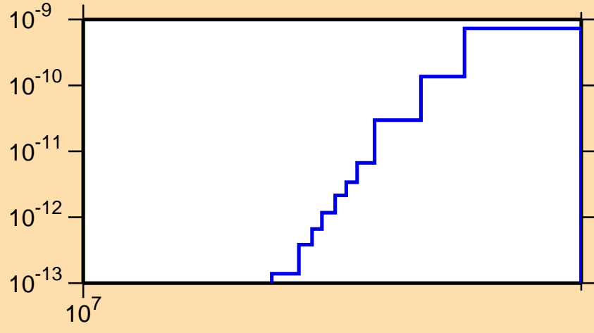
\sigma vs. E for ^{174}\text{Ta} (mt 45)
