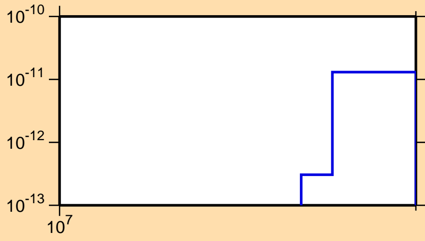
\sigma vs. E for ^{174}\text{Ta}(n,pd)
