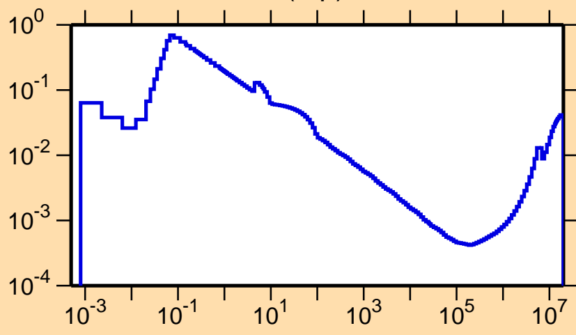
\sigma vs. E for ^{174}\text{Ta}(n,p)
