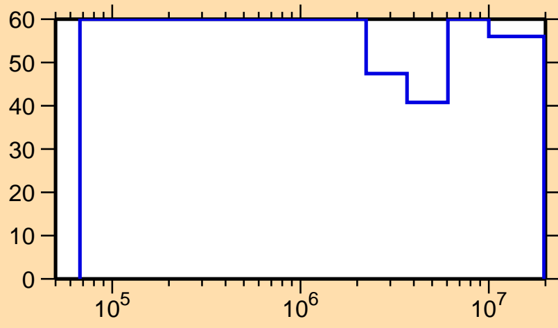
\Delta\sigma/\sigma vs. E for ^{174}\text{Ta}(n,n_1)
