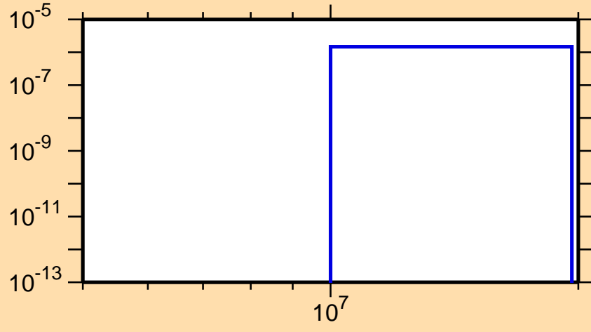
\sigma vs. E for ^{174}\text{Ta}(n,2n\alpha)
