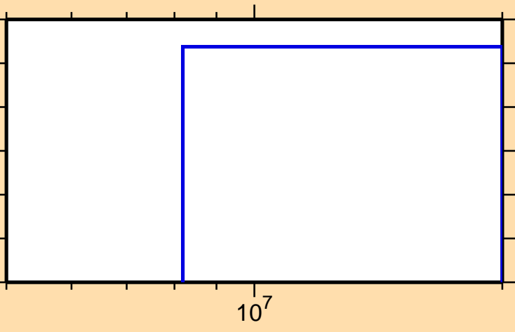
\sigma vs. E for ^{174}\text{Ta}(n,2np)
