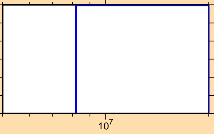
\sigma vs. E for ^{174}\text{Ta}(n,2n\alpha)
