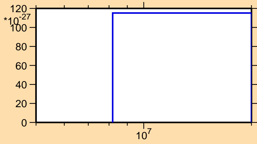
\sigma vs. E for ^{174}\text{Ta} (mt 42)
