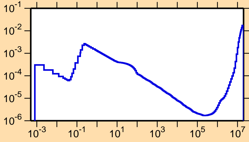
\sigma vs. E for ^{175}\text{Ta}(n,\alpha)
