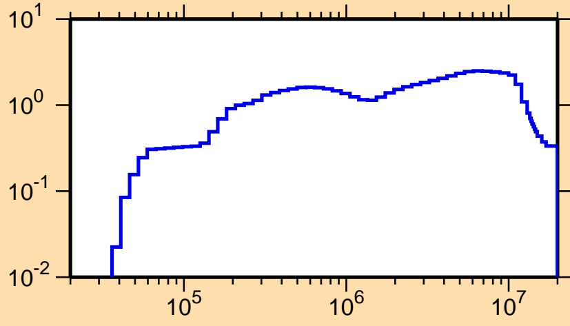
\sigma vs. E for ^{175}\text{Ta}(n,\text{inel.})
