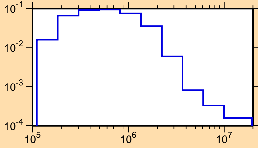
\sigma vs. E for ^{175}\text{Ta}(n,n_4)
