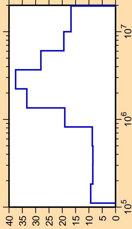
\Delta\sigma/\sigma vs. E for ^{175}\text{Ta}(n,n_4)
