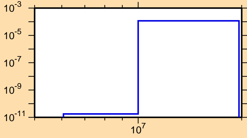
\sigma vs. E for ^{175}\text{Ta}(n,t)
