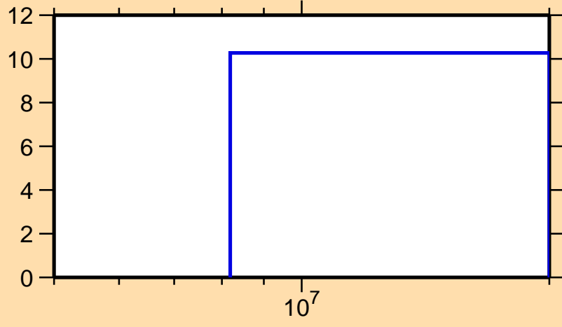
\Delta\sigma/\sigma vs. E for ^{175}\text{Ta}(n,\text{inel.})
