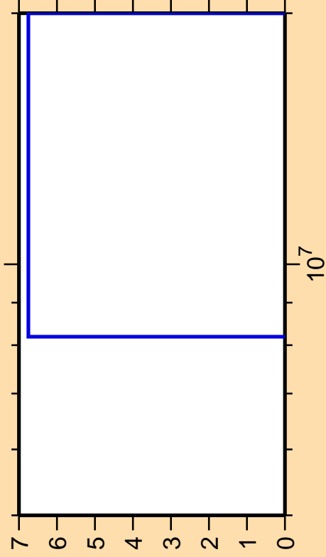
\Delta\sigma/\sigma vs. E for ^{175}\text{Ta}(n,2n)
