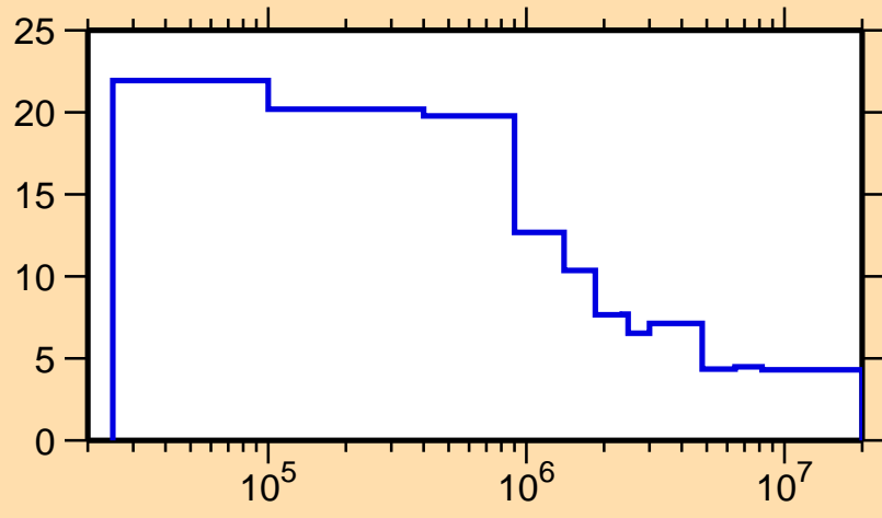
\Delta\sigma/\sigma vs. E for ^{175}\text{Ta}(n,\text{nonel.})
