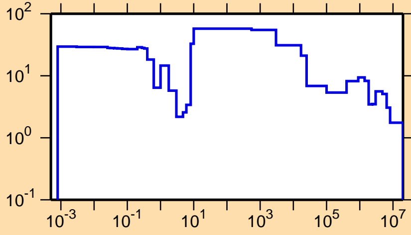
\Delta\sigma/\sigma vs. E for ^{175}\text{Ta}(n,\text{tot.})
