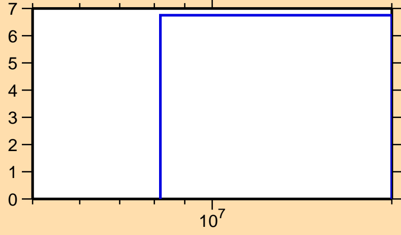
\Delta\sigma/\sigma vs. E for ^{175}\text{Ta}(n,2n)
