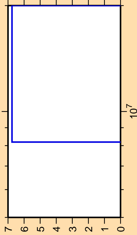
\Delta\sigma/\sigma vs. E for ^{175}\text{Ta}(n,2n)
