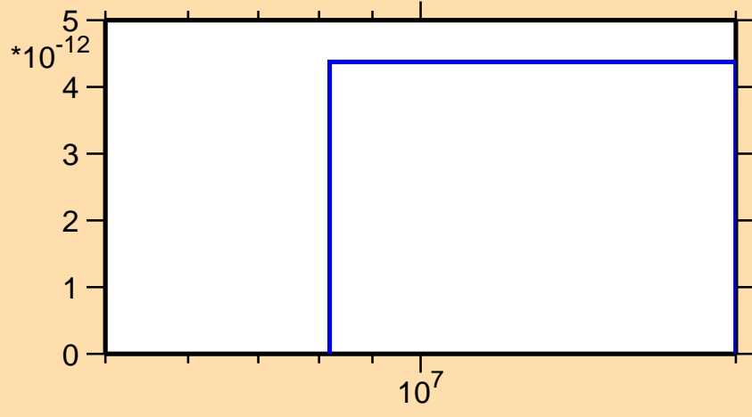
\sigma vs. E for ^{175}\text{Ta} (mt 45)
