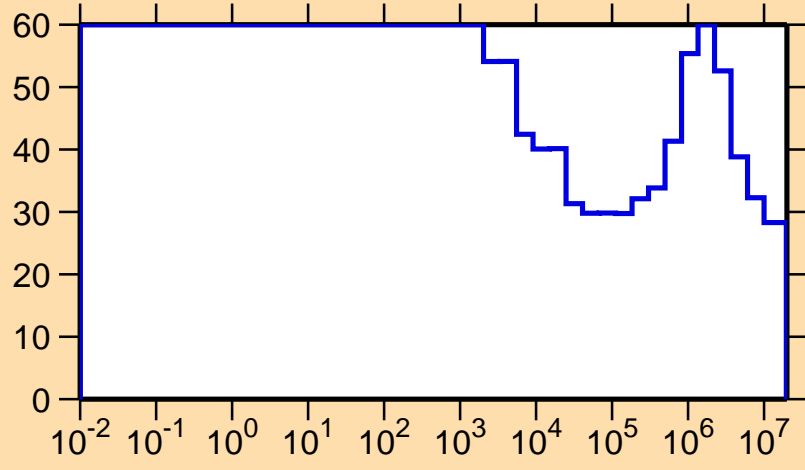
\Delta\sigma/\sigma vs. E for ^{176}\text{Ta}(n,p)
