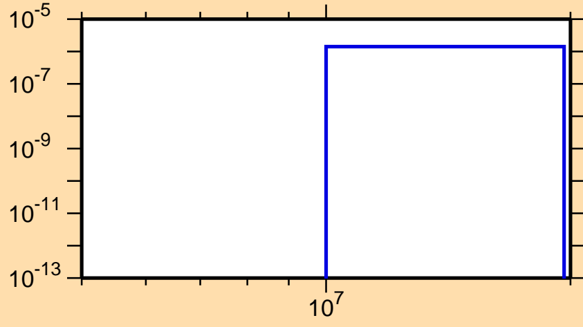
\sigma vs. E for ^{176}\text{Ta}(n,\text{nd})
