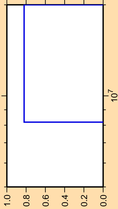
\Delta\sigma/\sigma vs. E for ^{176}\text{Ta}(\text{mt } 45)
