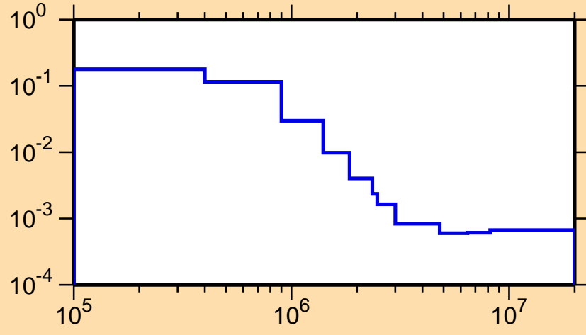
\sigma vs. E for ^{176}\text{Ta}(n,n_4)
