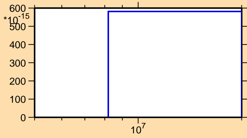
\sigma vs. E for ^{176}\text{Ta}(\text{mt } 45)
