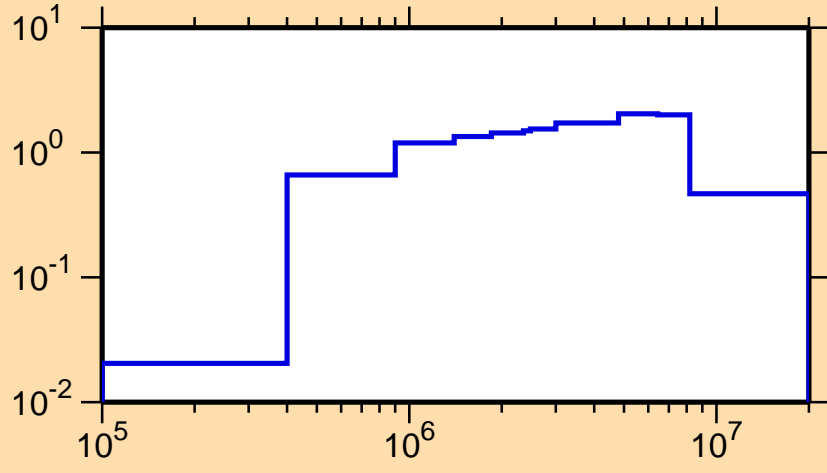
\sigma vs. E for ^{176}\text{Ta}(n,n\text{cont.})
