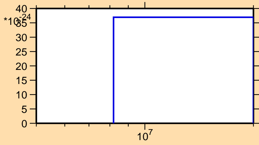
\sigma vs. E for ^{176}\text{Ta} (mt 42)
