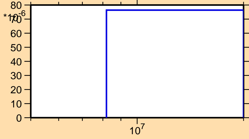
\sigma vs. E for ^{177}\text{Ta}(n,t)
