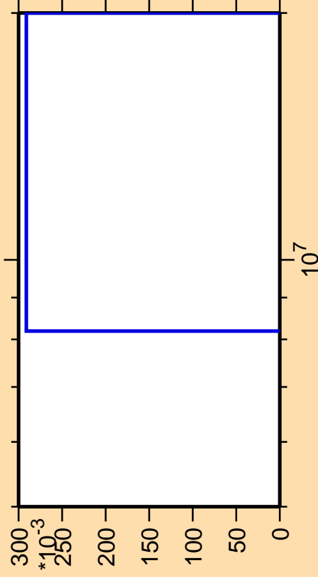
\Delta\sigma/\sigma vs. E for ^{177}\text{Ta}(\text{mt } 45)
