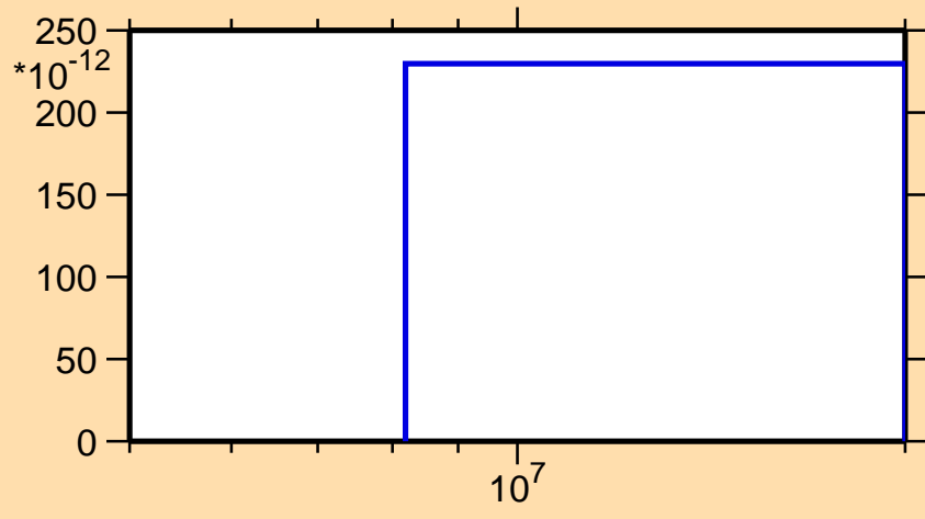
\sigma vs. E for ^{177}\text{Ta}(n,p\alpha)
