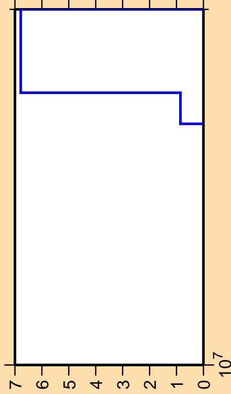
\Delta\sigma/\sigma vs. E for ^{178}\text{Ta}(\text{mt117})
