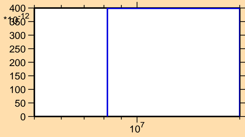
\sigma vs. E for ^{178}\text{Ta}(n,p\alpha)
