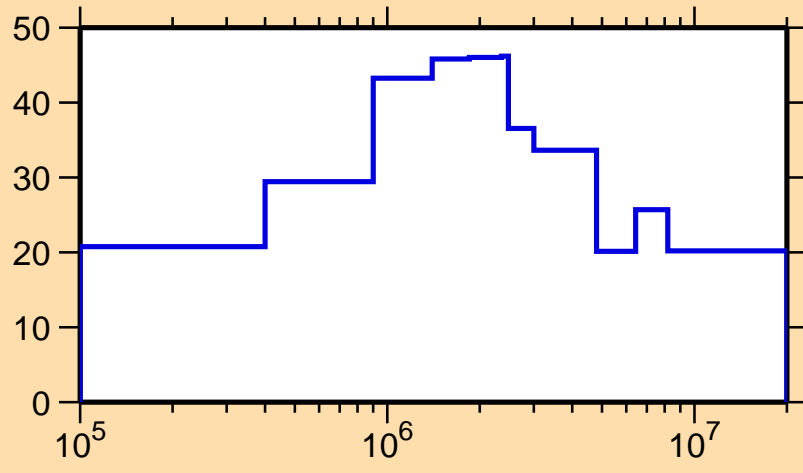
\Delta\sigma/\sigma vs. E for ^{178}\text{Ta}(n,n_1)
