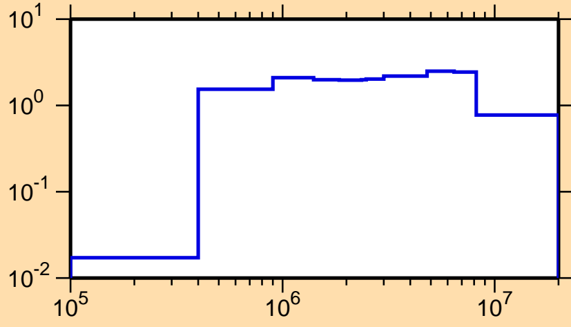
\sigma vs. E for ^{178}\text{Ta}(n,\text{inel.})
