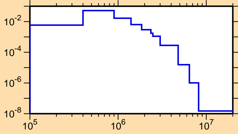
\sigma vs. E for ^{178}\text{Ta}(n,n_3)
