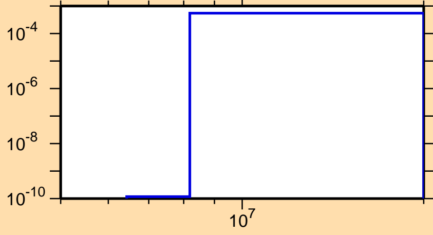
\sigma vs. E for ^{178}\text{Ta}(n,np)
