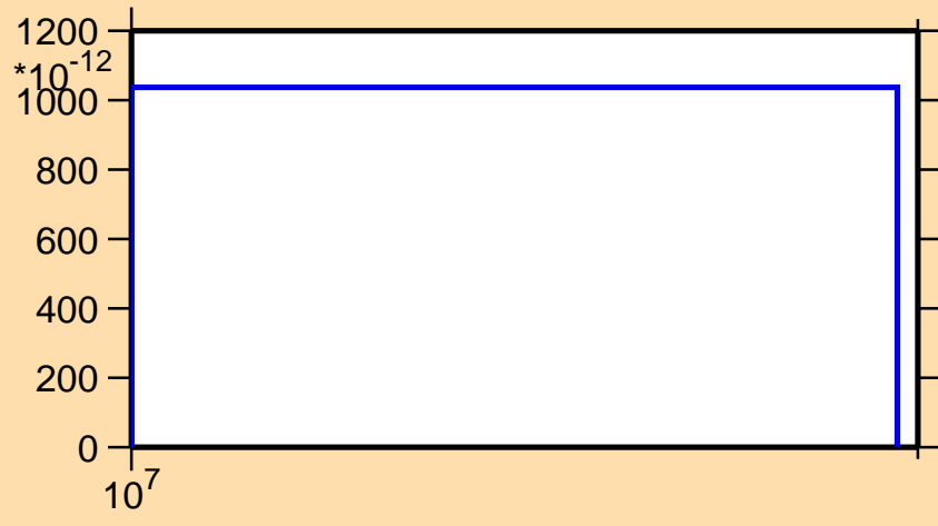
\sigma vs. E for ^{178}\text{Ta}(n,\text{He3})
