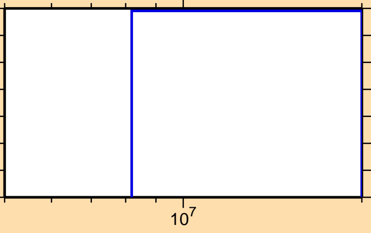
\sigma vs. E for ^{178}\text{Ta} (mt 42)
