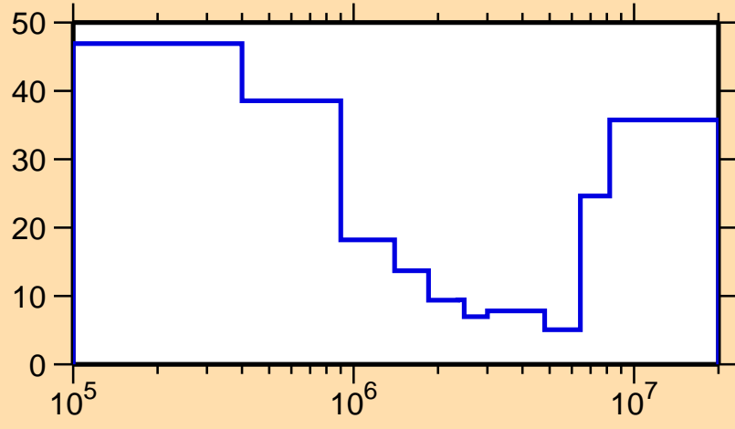
\Delta\sigma/\sigma vs. E for ^{178}\text{Ta}(n,n\text{cont.})
