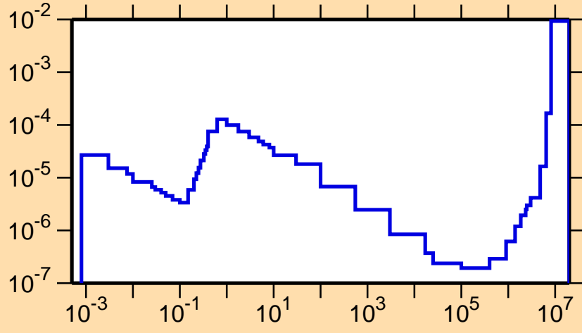
\sigma vs. E for ^{178}\text{Ta}(n,p)
