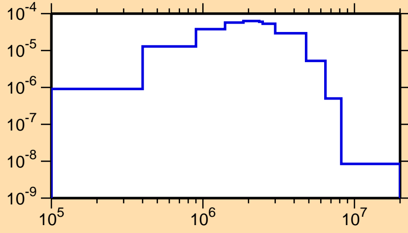
\sigma vs. E for ^{178}\text{Ta}(n,n_4)
