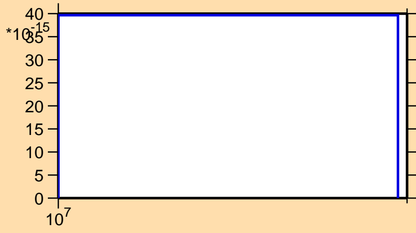
\sigma vs. E for ^{179}\text{Ta}(\text{mt117})
