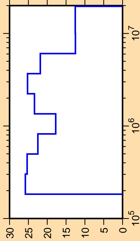
\Delta\sigma/\sigma vs. E for ^{179}\text{Ta}(n,n_4)
