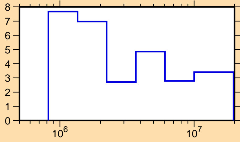
\Delta\sigma/\sigma vs. E for ^{179}\text{Ta}(n, el.)
