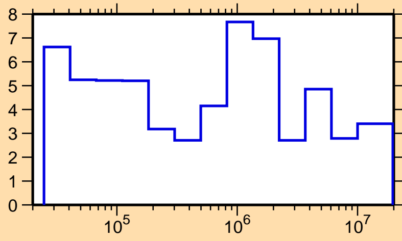
\Delta\sigma/\sigma vs. E for ^{179}\text{Ta}(n,\text{el.})
