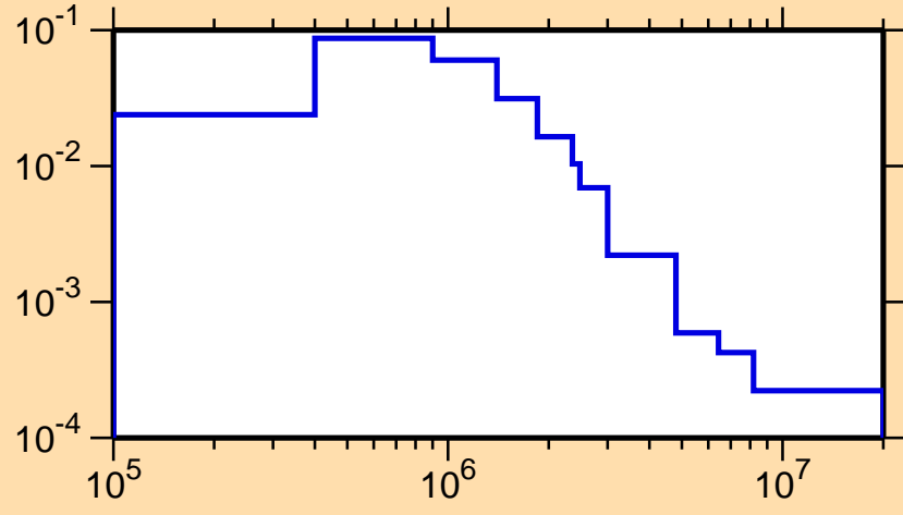
\sigma vs. E for ^{179}\text{Ta}(n,n_3)
