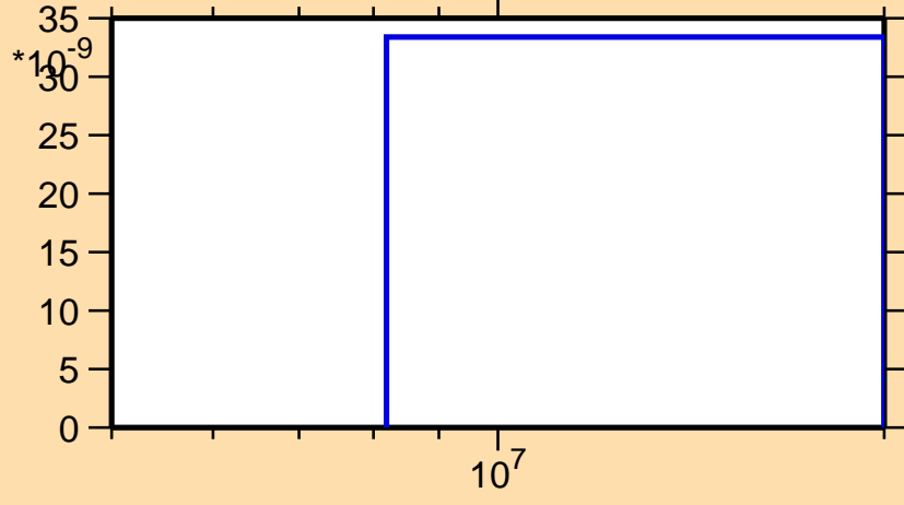
\sigma vs. E for ^{179}\text{Ta}(n,\text{nd})
