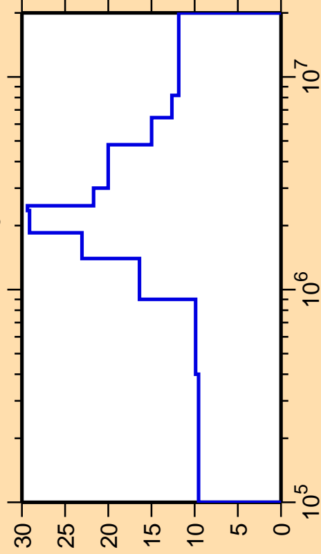
\Delta\sigma/\sigma vs. E for ^{179}\text{Ta}(n,n_3)
