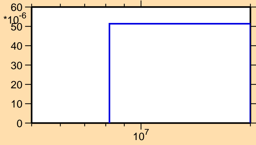
\sigma vs. E for ^{179}\text{Ta}(n,t)
