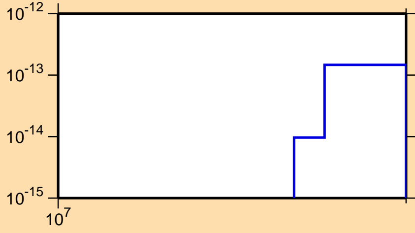
\sigma vs. E for ^{180}\text{Ta}(\text{mt117})
