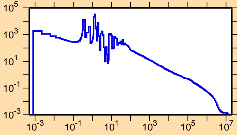
\sigma vs. E for ^{180}\text{Ta}(n,\gamma)
