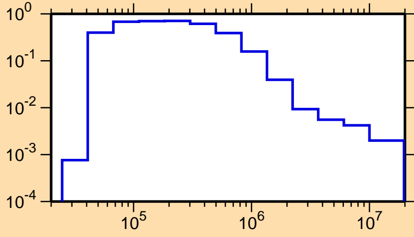
\sigma vs. E for ^{180}\text{Ta}(n,n_1)
