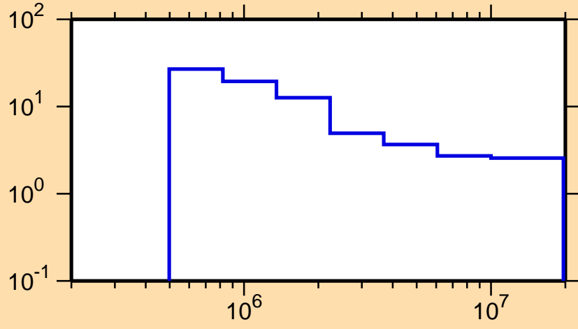
\Delta\sigma/\sigma vs. E for ^{180}\text{Ta}(n,n\text{onel.})
