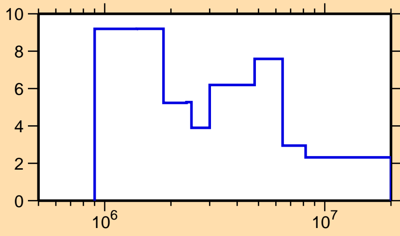
\Delta\sigma/\sigma vs. E for ^{180}\text{Ta}(n,el.)
