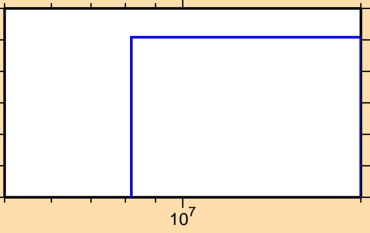
\sigma vs. E for ^{180}\text{Ta}(n,t)
