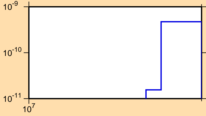
\sigma vs. E for ^{181}\text{Ta}(n,\text{He3})
