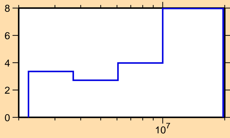
\Delta\sigma/\sigma vs. E for ^{181}\text{Ta}(n,n\text{cont.})
