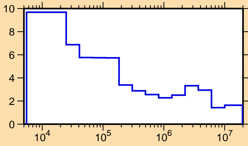
\Delta\sigma/\sigma vs. E for ^{181}\text{Ta}(n,\text{el.})
