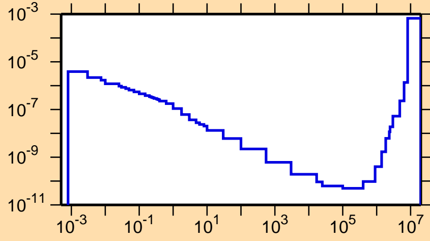
\sigma vs. E for ^{181}\text{Ta}(n,\alpha)
