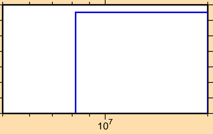
\sigma vs. E for ^{181}\text{Ta}(n,p\alpha)
