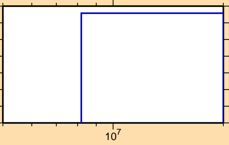
\sigma vs. E for ^{181}\text{Ta}(n,t)
