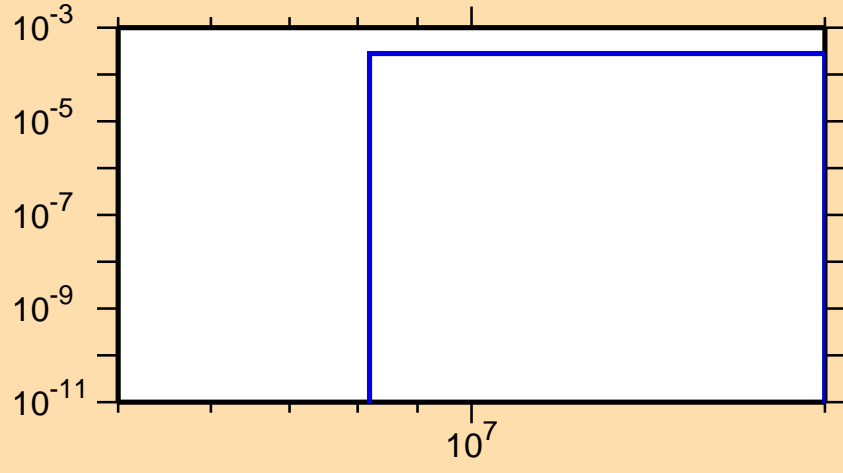
\sigma vs. E for ^{182}\text{Ta}(n,np)
