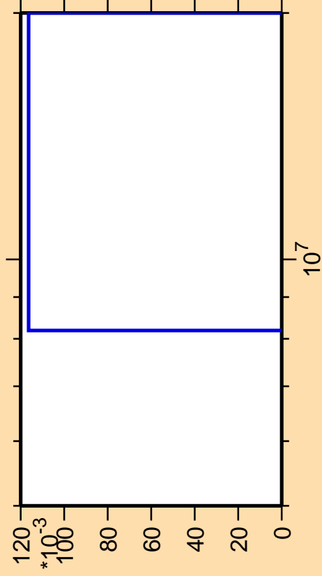
\Delta\sigma/\sigma vs. E for ^{182}\text{Ta}(n,p\alpha)
