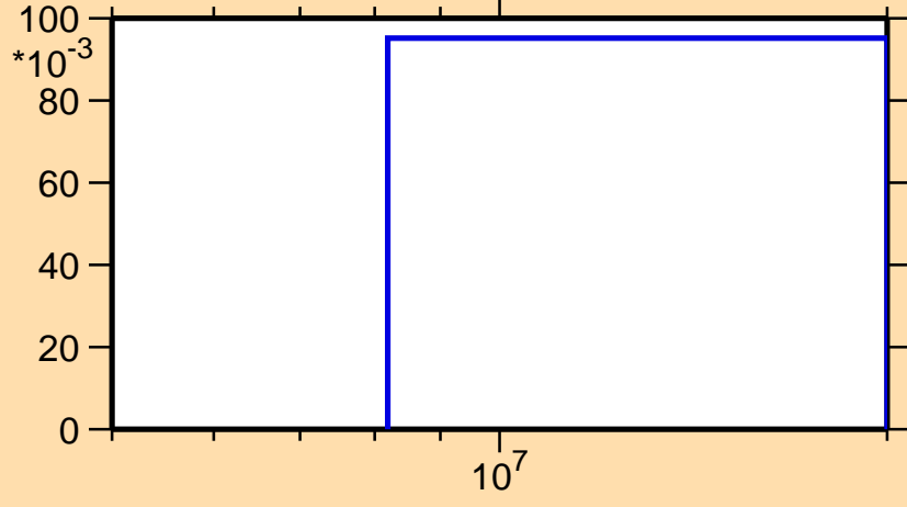
\sigma vs. E for ^{182}\text{Ta}(n,3n)
