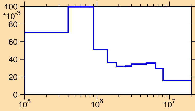
\sigma vs. E for ^{182}\text{Ta}(n,n_4)
