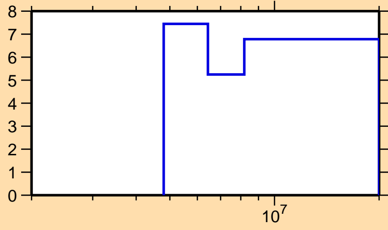
\Delta\sigma/\sigma vs. E for ^{182}\text{Ta}(n,2n)
