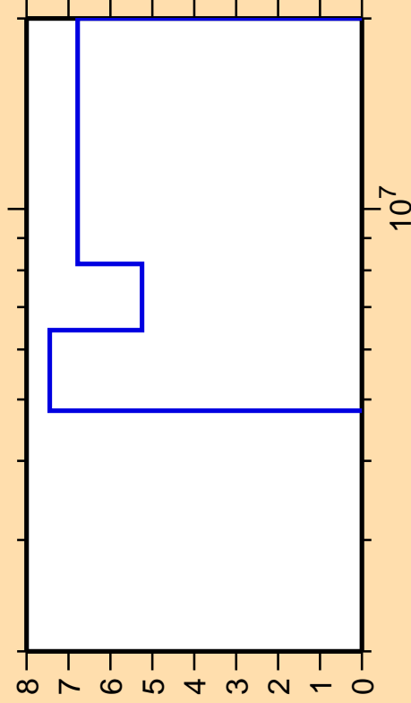
\Delta\sigma/\sigma vs. E for ^{182}\text{Ta}(n,2n)
