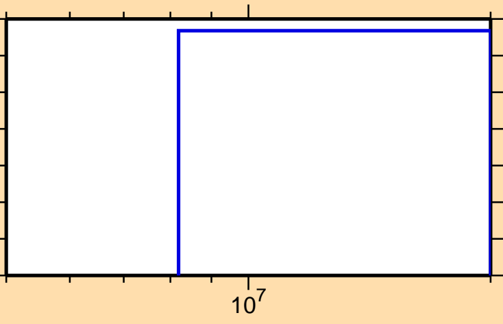
\sigma vs. E for ^{182}\text{Ta}(n,2np)
