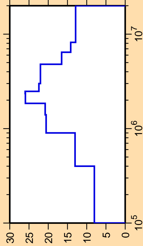
\Delta\sigma/\sigma vs. E for ^{182}\text{Ta}(n,n_4)
