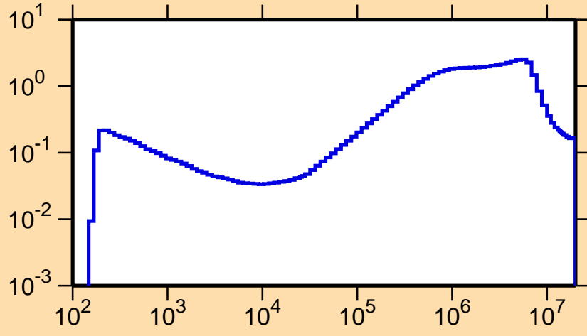
\sigma vs. E for ^{182}\text{Ta}(n,\text{inel.})
