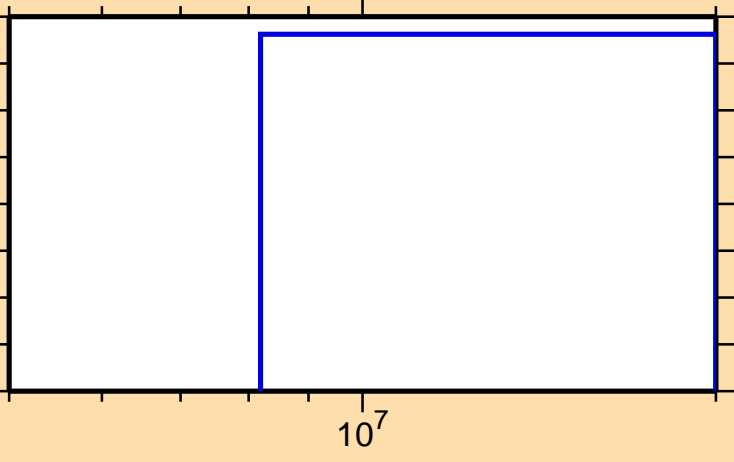
\sigma vs. E for ^{182}\text{Ta}(n,2n\alpha)
