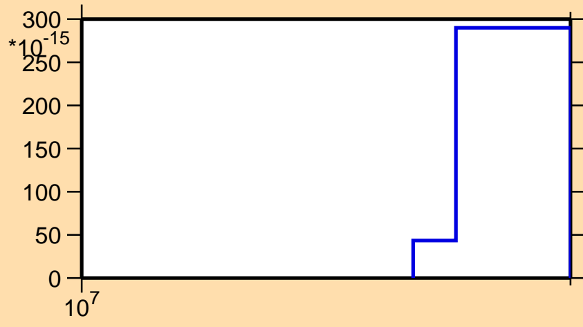
\sigma vs. E for ^{183}\text{Ta}(n,p\alpha)
