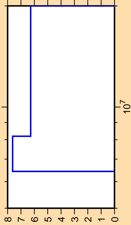
\Delta\sigma/\sigma vs. E for ^{183}\text{Ta}(n,2n)
