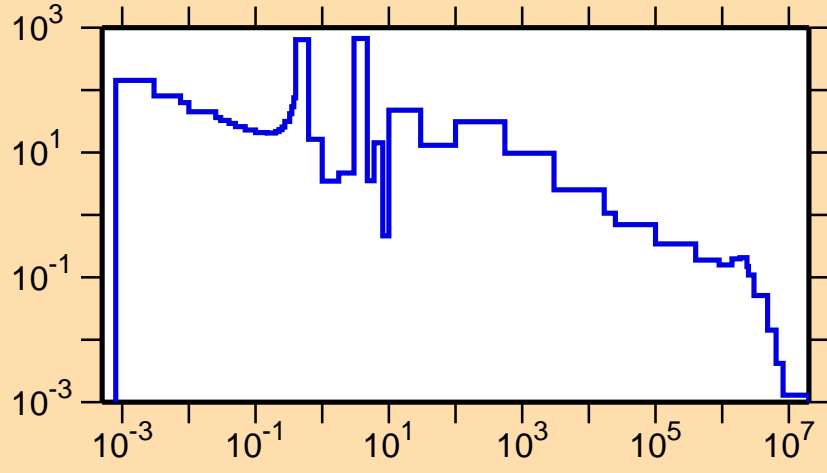
\sigma vs. E for ^{183}\text{Ta}(n,\gamma)
