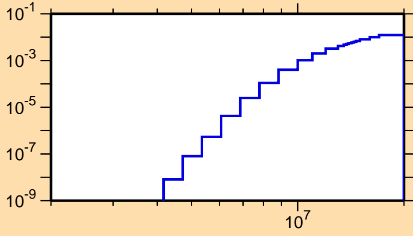
\sigma vs. E for ^{184}\text{Ta}(n,p)
