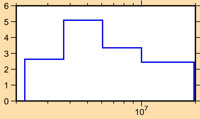
\Delta\sigma/\sigma vs. E for ^{184}\text{Ta}(n,\text{el.})
