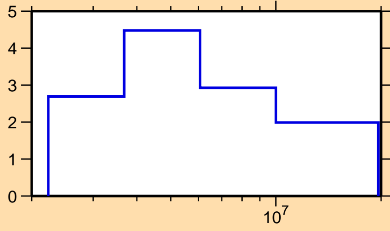
\Delta\sigma/\sigma vs. E for ^{184}\text{Ta}(n,\text{tot.})
