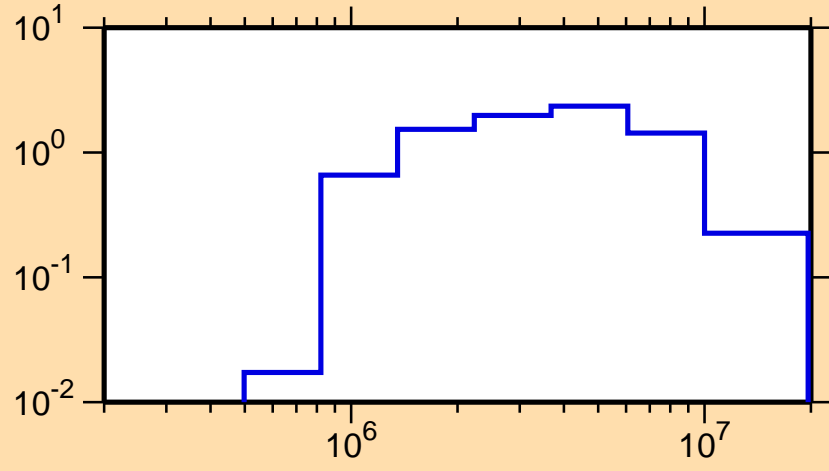
\sigma vs. E for ^{184}\text{Ta}(n,n\text{cont.})
