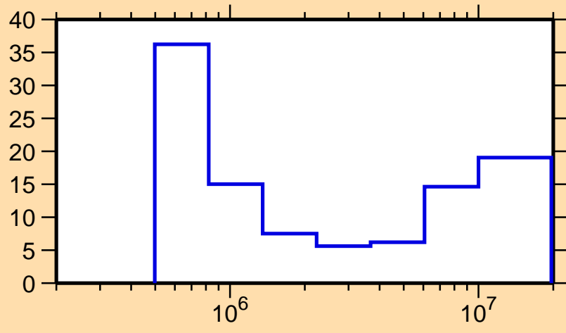
\Delta\sigma/\sigma vs. E for ^{184}\text{Ta}(n,n\text{cont.})
