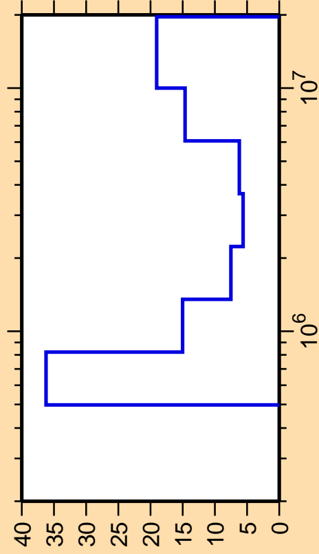
\Delta\sigma/\sigma vs. E for ^{184}\text{Ta}(n,\text{ncont.})
