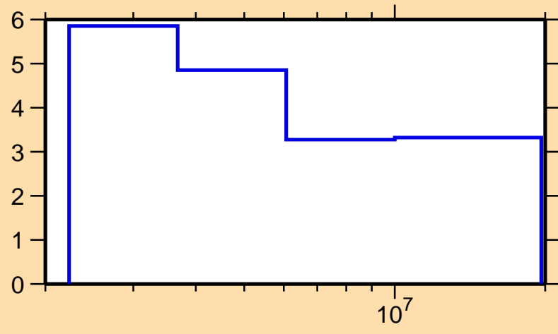
\Delta\sigma/\sigma vs. E for ^{184}\text{Ta}(n,\text{nonel.})
