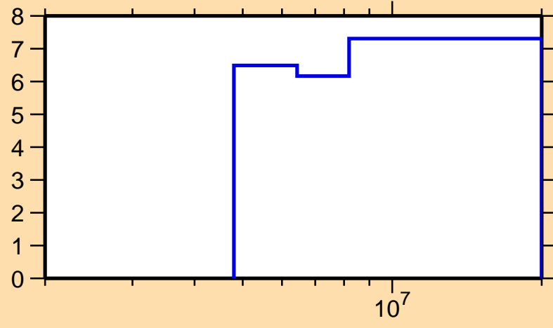
\Delta\sigma/\sigma vs. E for ^{184}\text{Ta}(n,2n)
