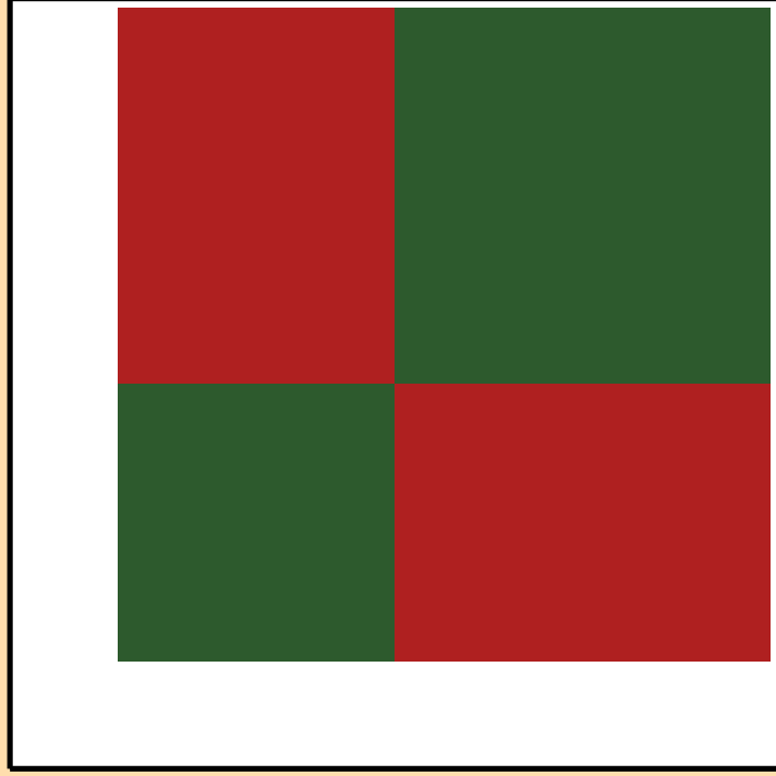
\sigma vs. E for ^{185}\text{Ta}(n,2n)
