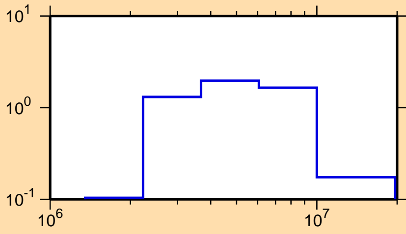
\sigma vs. E for ^{185}\text{Ta}(n,n\text{cont.})
