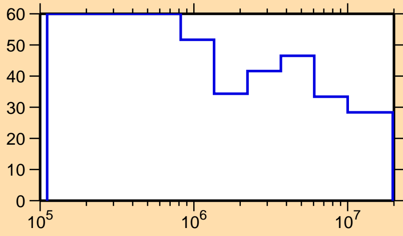
\Delta\sigma/\sigma vs. E for ^{185}\text{Ta}(n,n_1)
