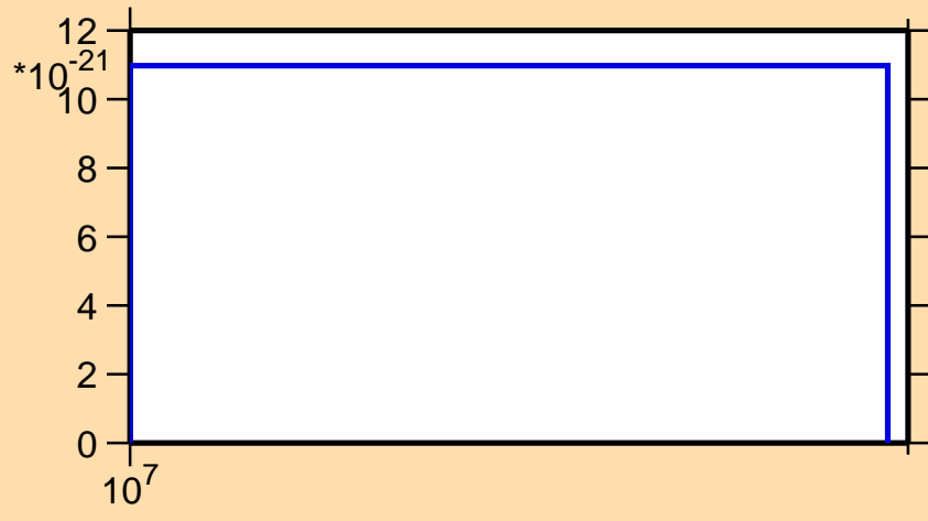
\sigma vs. E for ^{185}\text{Ta} (mt 42)
