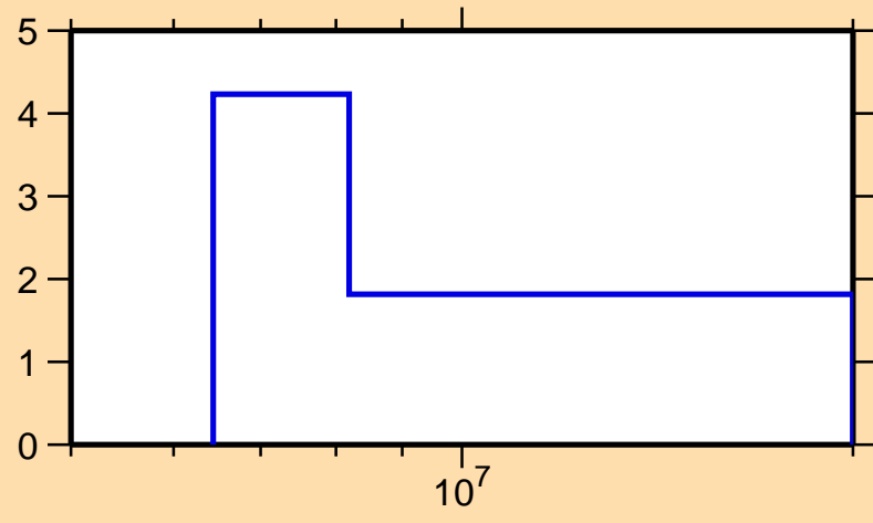
\Delta\sigma/\sigma vs. E for ^{185}\text{Ta}(n,\text{tot.})
