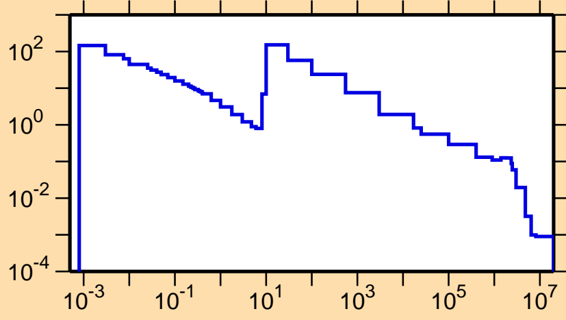
\sigma vs. E for ^{185}\text{Ta}(n,\gamma)
