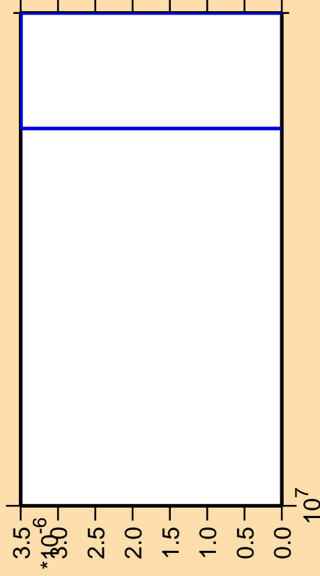
\Delta\sigma/\sigma vs. E for ^{186}\text{Ta} (mt 42)
