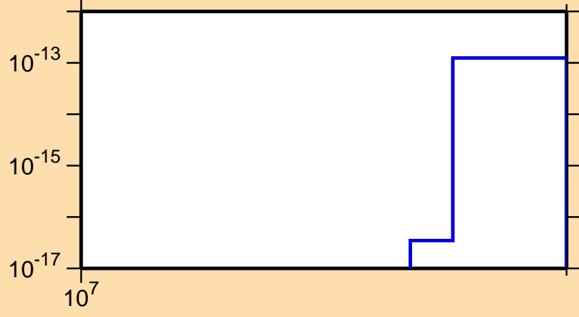
\sigma vs. E for ^{186}\text{Ta}(n,3n\alpha)
