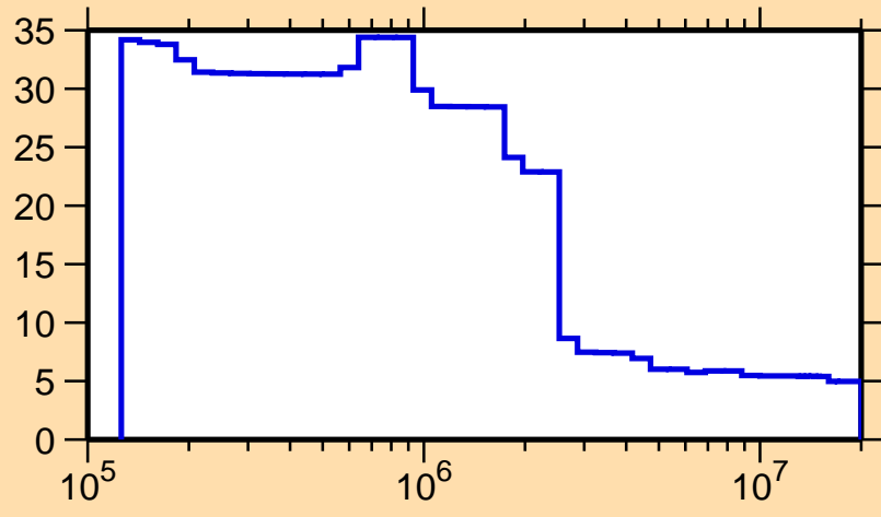
\Delta\sigma/\sigma vs. E for ^{186}\text{Ta}(n,\text{nonel.})
