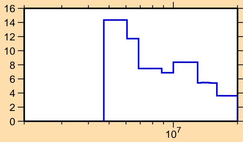
\Delta\sigma/\sigma vs. E for ^{186}\text{Ta}(n,\text{el.})
