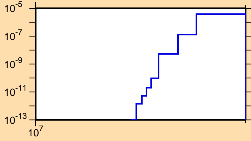
\sigma vs. E for ^{186}\text{Ta}(n,nt)
