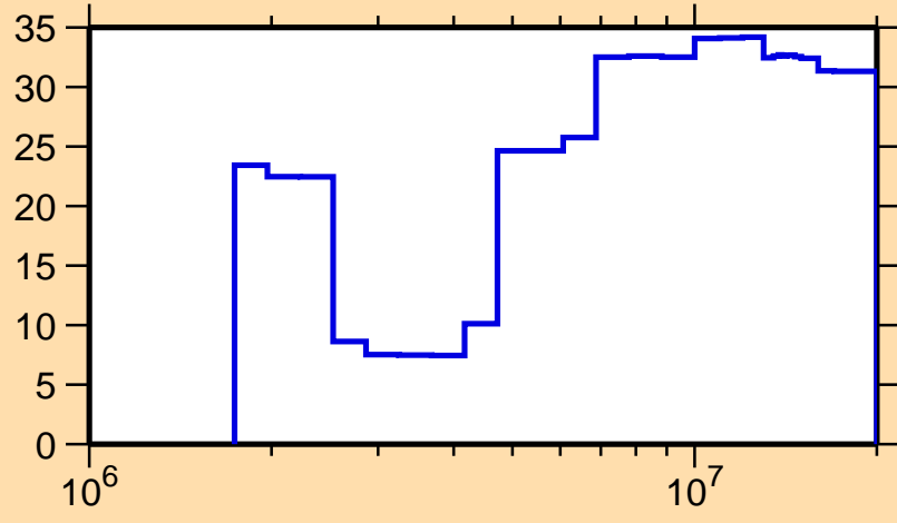
\Delta\sigma/\sigma vs. E for ^{186}\text{Ta}(n,n\text{cont.})
