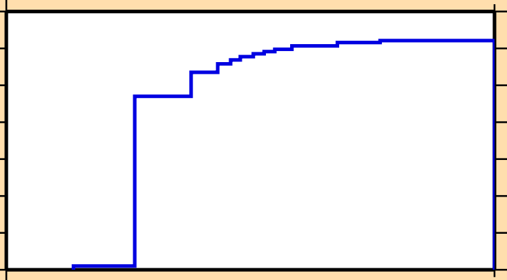
\sigma vs. E for ^{186}\text{Ta}(n,3n)
