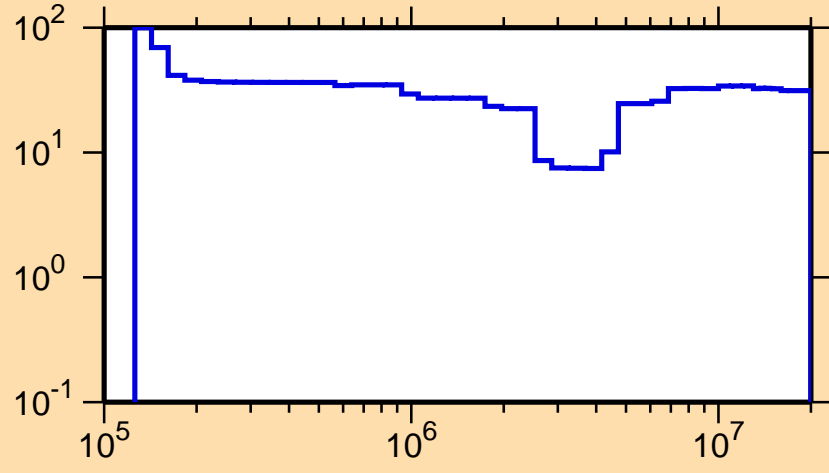
\Delta\sigma/\sigma vs. E for ^{186}\text{Ta}(n,n\text{cont.})
