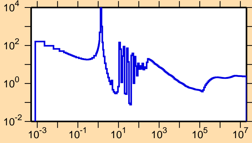
\sigma vs. E for ^{186}\text{Ta}(n,\text{nonel.})
