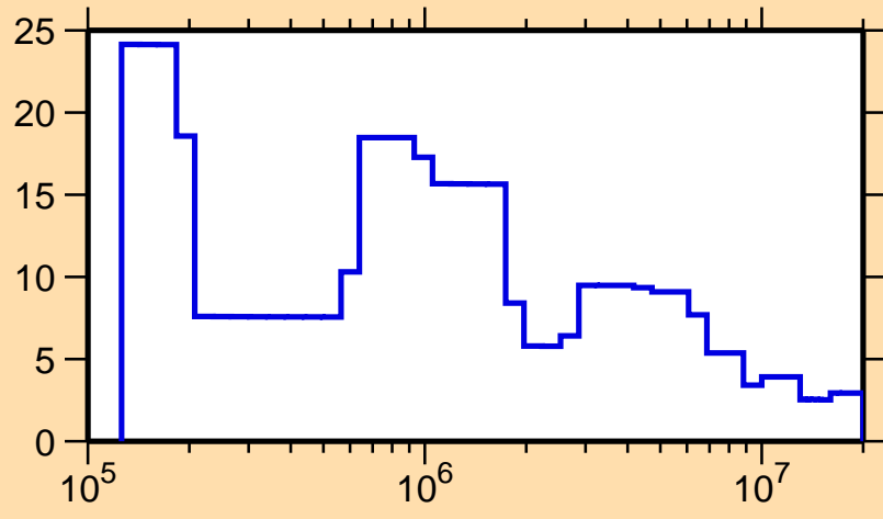
\Delta\sigma/\sigma vs. E for ^{186}\text{Ta}(n,\text{tot.})
