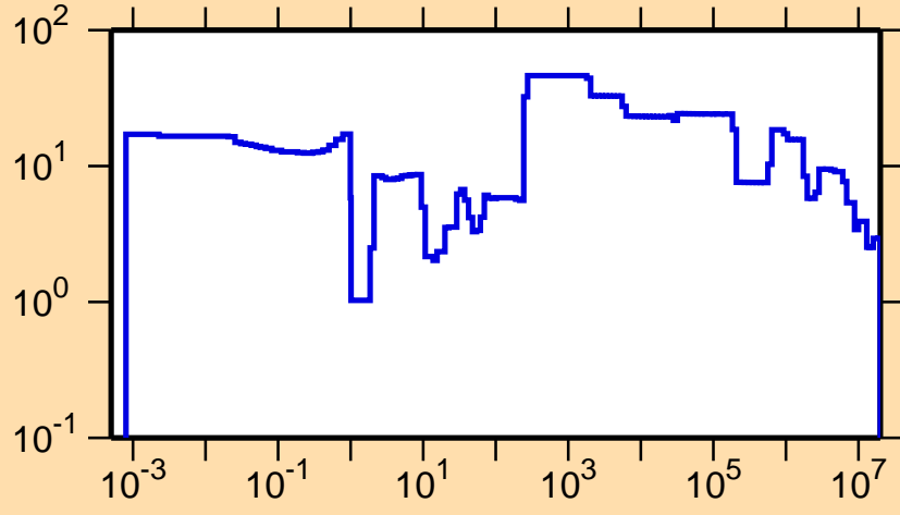
\Delta\sigma/\sigma vs. E for ^{186}\text{Ta}(n,\text{tot.})
