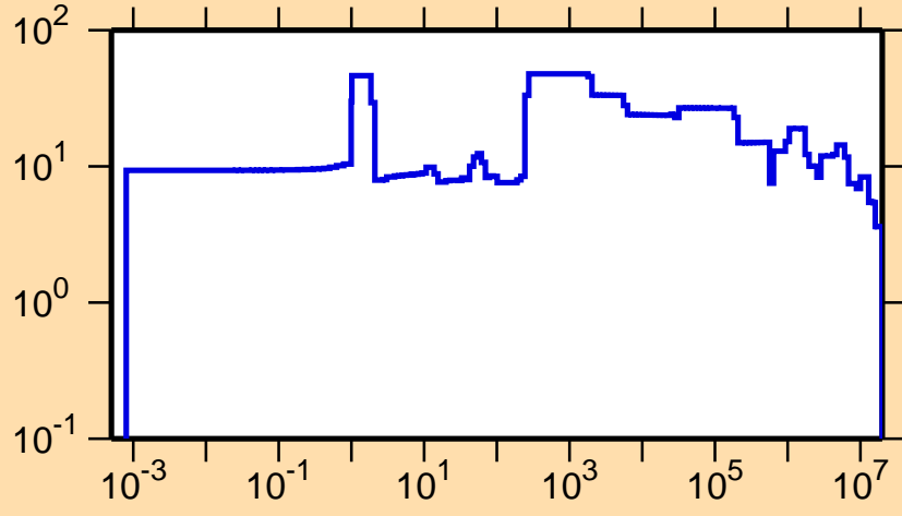
\Delta\sigma/\sigma vs. E for ^{186}\text{Ta}(n,\text{el.})
