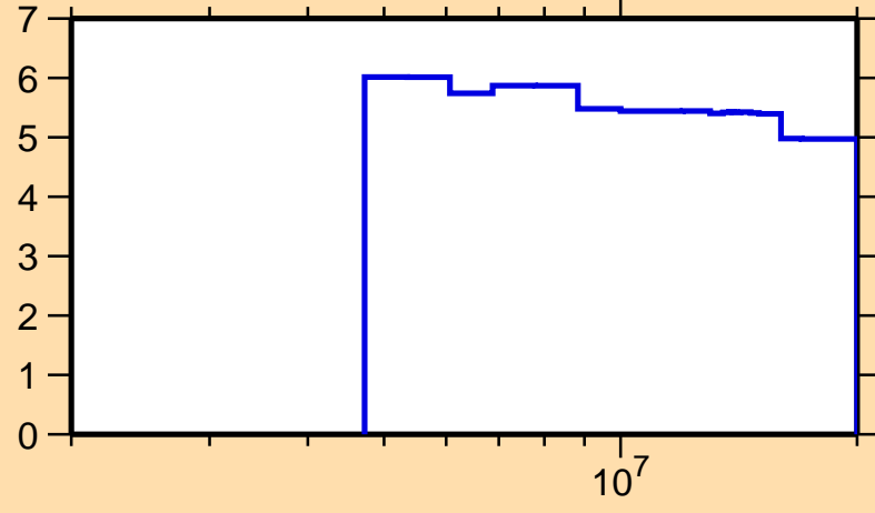
\Delta\sigma/\sigma vs. E for ^{186}\text{Ta}(n,\text{nonel.})
