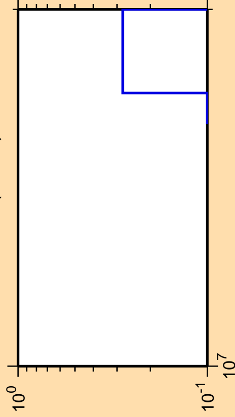
\Delta\sigma/\sigma vs. E for ^{186}\text{Ta}(n,3n\alpha)
