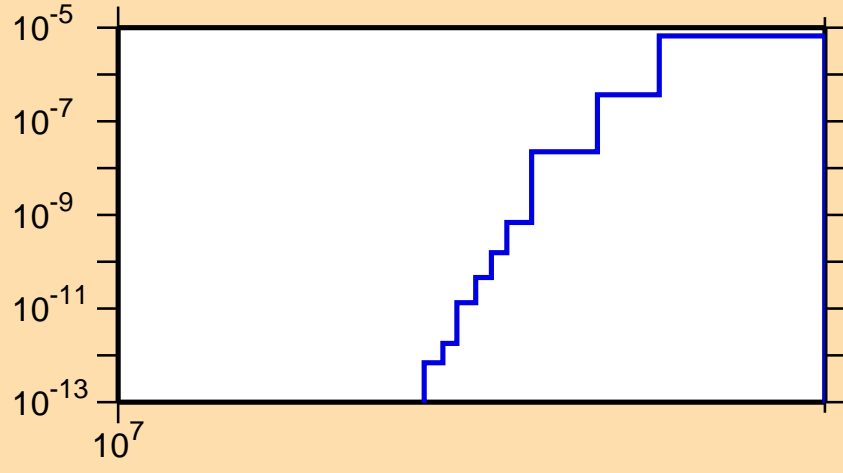
\sigma vs. E for ^{186}\text{Ta}(n,\text{nd})
