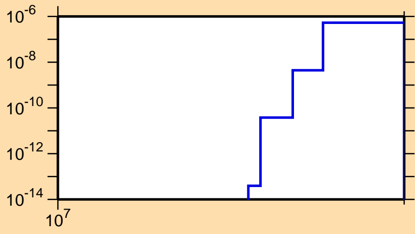
\sigma vs. E for ^{186}\text{Ta}(n,2np)
