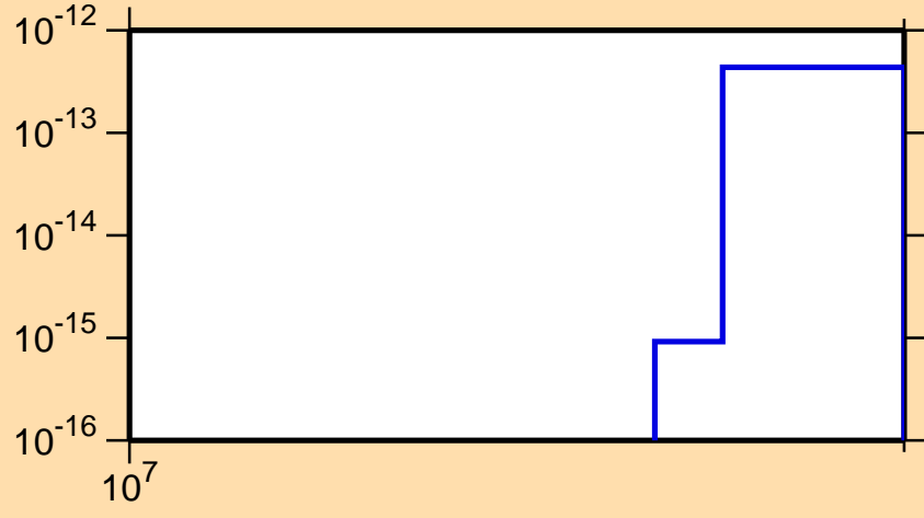
\sigma vs. E for ^{186}\text{Ta}(n,\text{He3})
