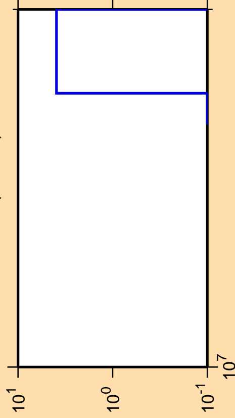
\Delta\sigma/\sigma vs. E for ^{186}\text{Ta}(n,\text{He3})
