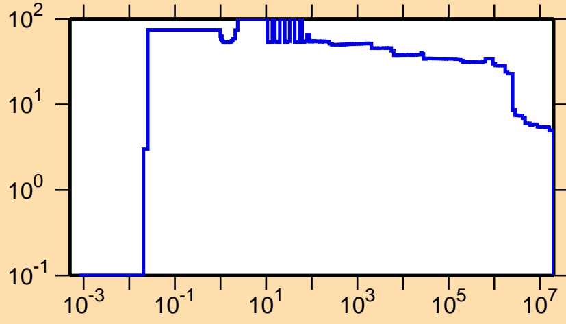
\Delta\sigma/\sigma vs. E for ^{186}\text{Ta}(n,\text{nonel.})
