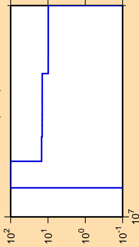
\Delta\sigma/\sigma vs. E for ^{186}\text{Ta}(n,3n)
