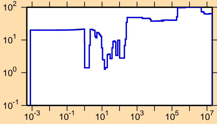
\Delta\sigma/\sigma vs. E for ^{186}\text{Ta}(n,\gamma)
