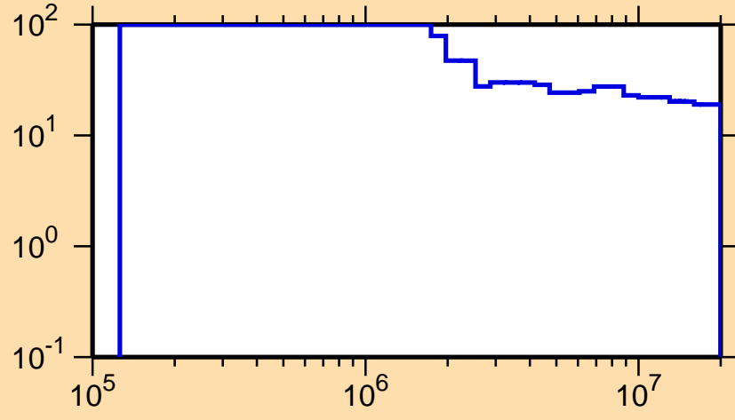
\Delta\sigma/\sigma vs. E for ^{186}\text{Ta}(n,n_1)
