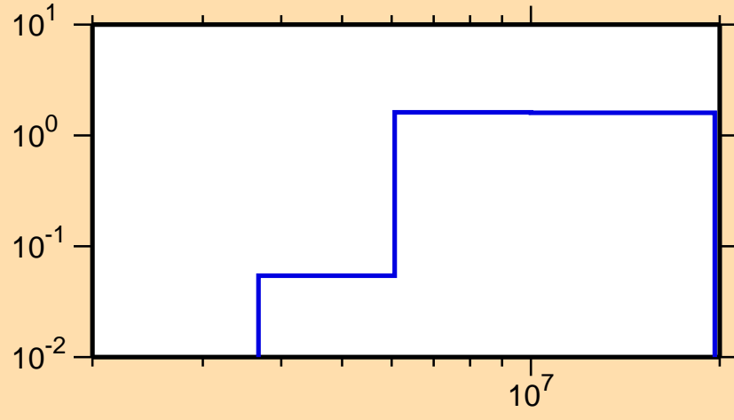
\sigma vs. E for ^{186}\text{Ta}(n,2n)
