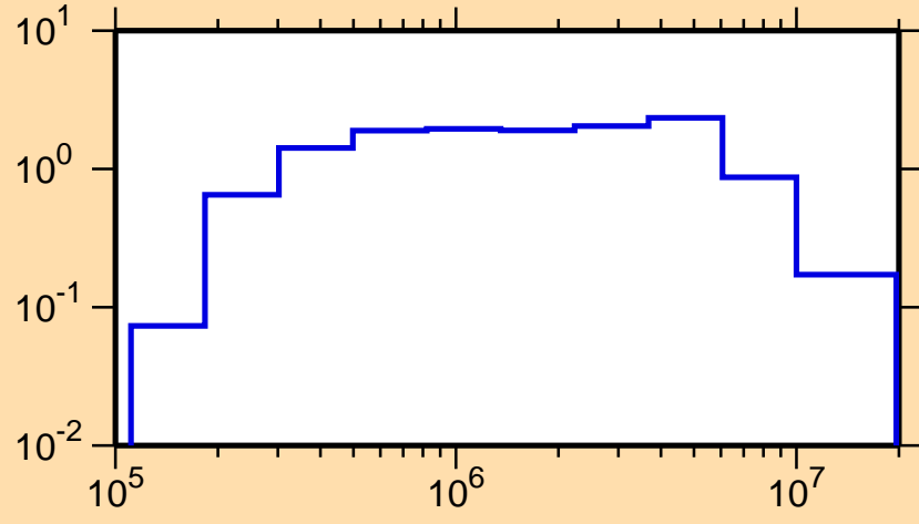
\sigma vs. E for ^{186}\text{Ta}(n,n\text{cont.})
