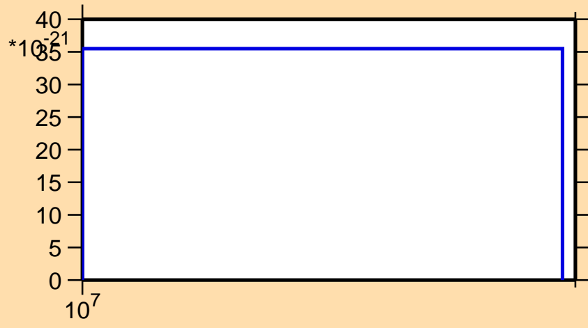
\sigma vs. E for ^{186}\text{Ta} (mt 42)
