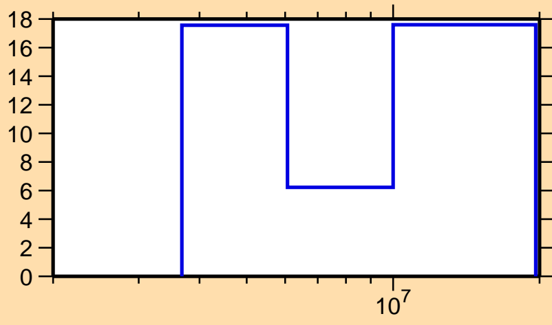
\Delta\sigma/\sigma vs. E for ^{186}\text{Ta}(n,2n)
