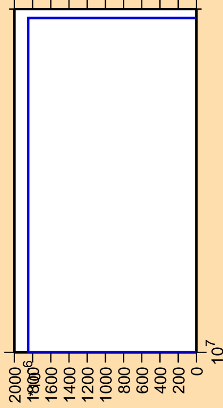
\Delta\sigma/\sigma vs. E for ^{186}\text{Ta}(n,3n\alpha)
