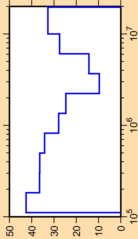
\Delta\sigma/\sigma vs. E for ^{186}\text{Ta}(n,n\text{cont.})
