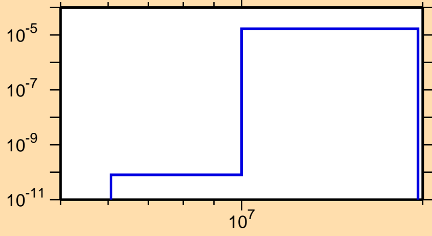
\sigma vs. E for ^{186}\text{Ta}(n,n\alpha)
