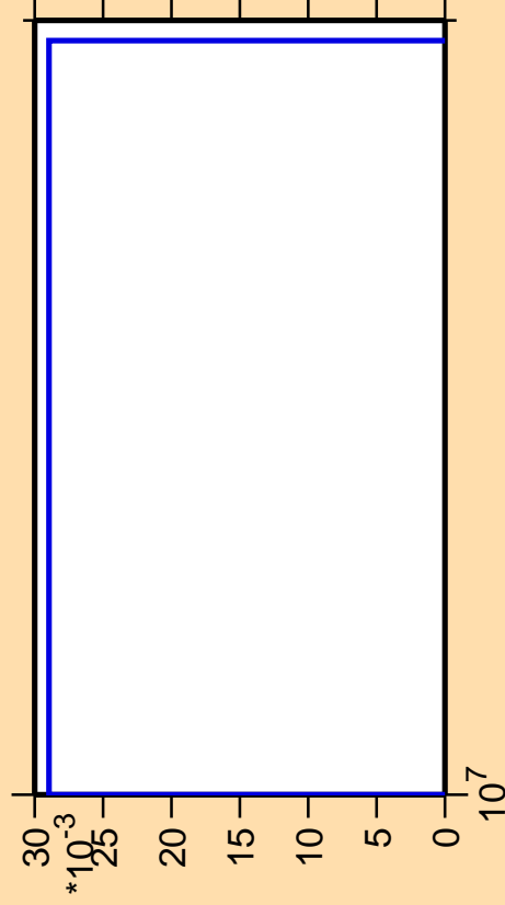
\Delta\sigma/\sigma vs. E for ^{186}\text{Ta}(n,\text{He3})
